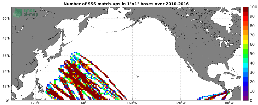
Figure 4: Number of SSS match-ups between TSG (LEGOS-DM) SSS and the SMOS SSS L3 v3 Monthly (ICDC) SSS product for the North Pacific Ocean Pi-MEP region over 1°x1° boxes and for the full satellite product period.
