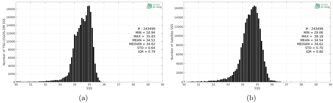
Figure 2: Histograms of SSS from TSG-LEGOS-DM (a) and SMOS-L3-ICDC-V3-MONTHLY-0.5DEG (b) considering all match-up pairs per bins of 0.1 over the North Pacific Ocean Pi-MEP region and for the full satellite product period.
