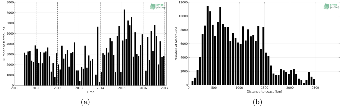
Figure 1: Number of match-ups between TSG-LEGOS-DM and SMOS-L3-ICDC-V3-MONTHLY-0.5DEG SSS as a function of time (a) and as function of the distance to coast (b) over the North Pacific Ocean Pi-MEP region and for the full satellite product period.
