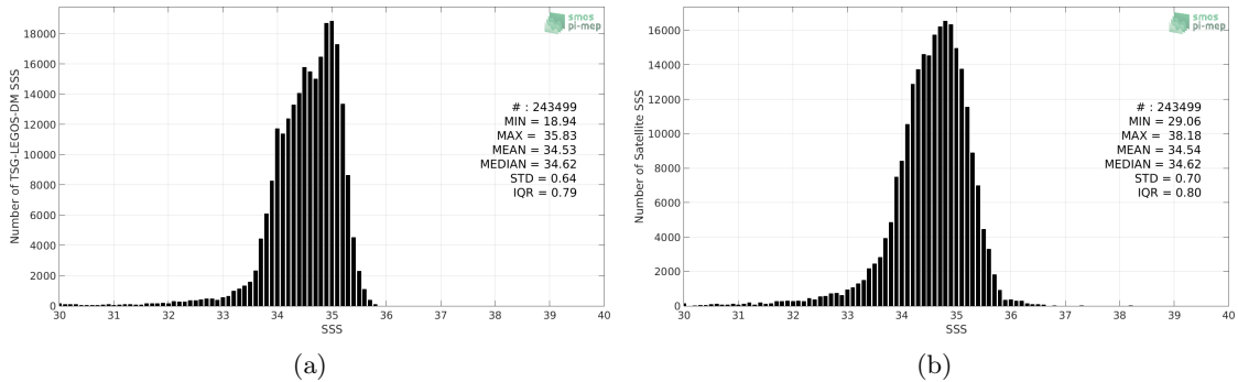
Figure 2: Histograms of SSS from TSG-LEGOS-DM (a) and SMOS-L3-ICDC-V3-MONTHLY-0.5DEG (b) considering all match-up pairs per bins of 0.1 over the North Pacific Ocean Pi-MEP region and for the full satellite product period.
