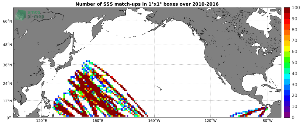
Figure 4: Number of SSS match-ups between TSG-LEGOS-DM SSS and the SMOS-L3-ICDC-V3-MONTHLY-0.5DEG SSS product for the North Pacific Ocean Pi-MEP region over 1°x1° boxes and for the full satellite product period.
