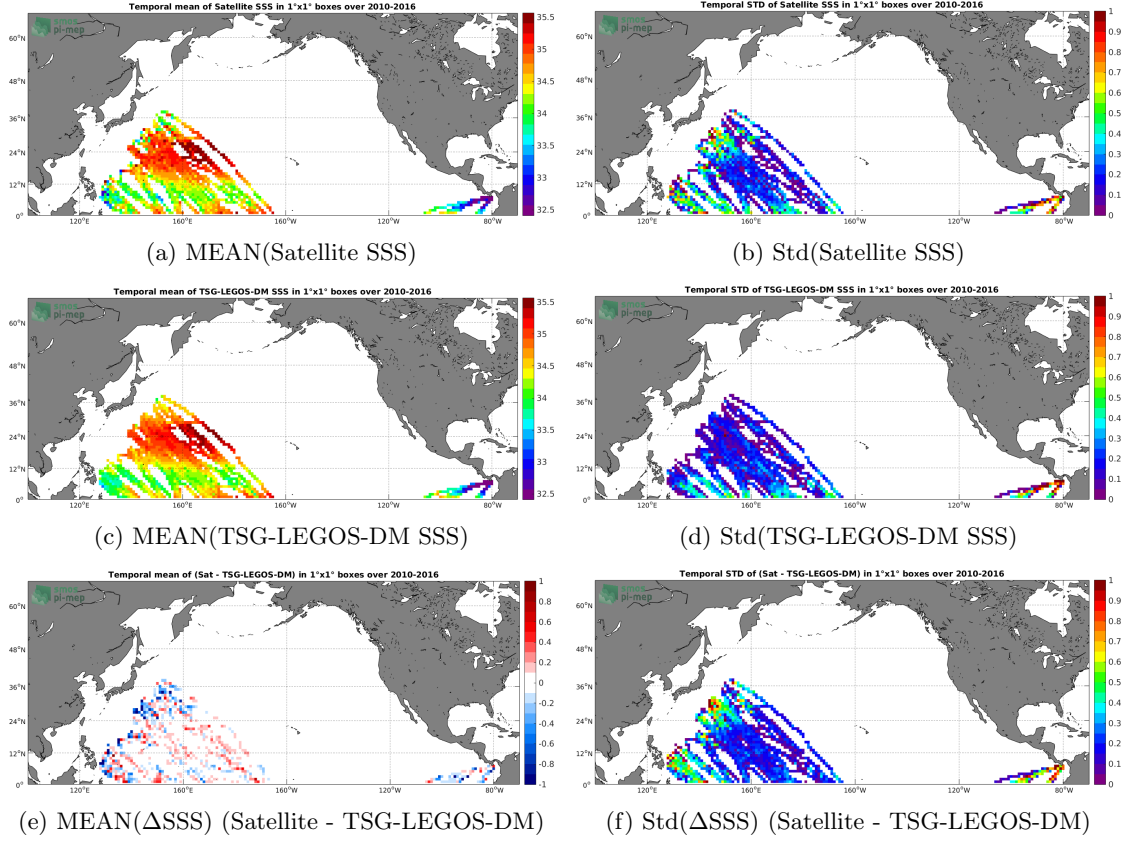
Figure 6: Temporal mean (left) and Std (right) of SSS from SMOS-L3-ICDC-V3-MONTHLY-0.5DEG (top), TSG-LEGOS-DM (middle), and of \Delta SSS (Satellite - TSG-LEGOS-DM). Only match-up pairs are used to generate these maps.
