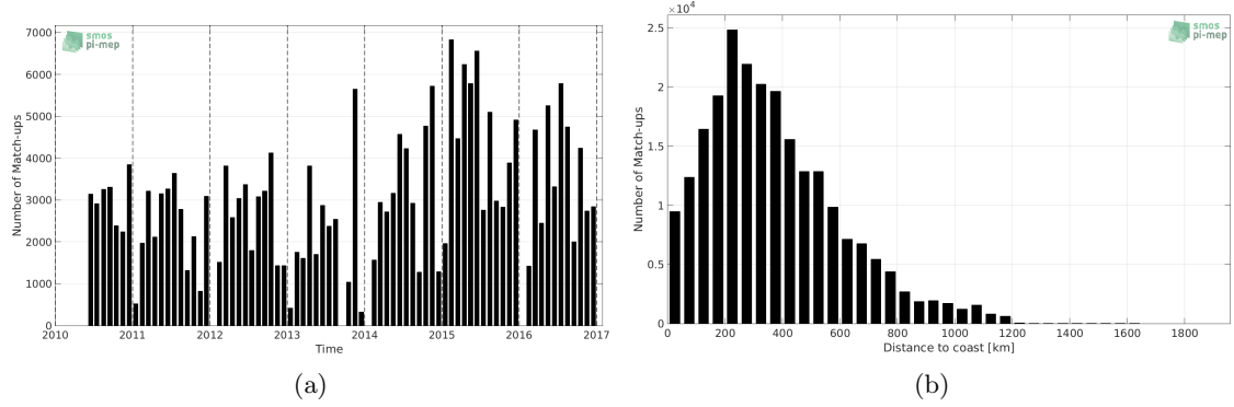
Figure 1: Number of match-ups between TSG-LEGOS-DM and SMOS-L3-ICDC-V3-MONTHLY-0.5DEG SSS as a function of time (a) and as function of the distance to coast (b) over the North Pacific Ocean Pi-MEP region and for the full satellite product period.
