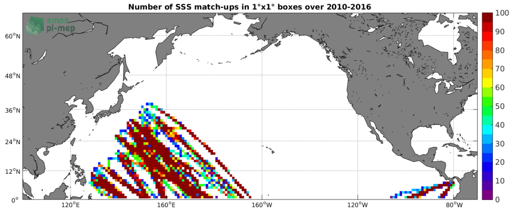
Figure 4: Number of SSS match-ups between TSG-LEGOS-DM SSS and the SMOS-L3-ICDC-V3-MONTHLY-0.5DEG SSS product for the North Pacific Ocean Pi-MEP region over 1^\circ \times 1^\circ boxes and for the full satellite product period.
