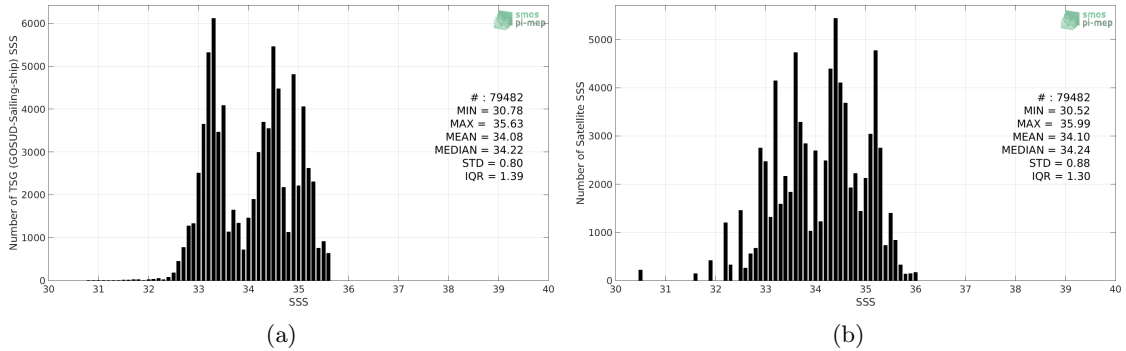
Figure 2: Histograms of SSS from TSG (GOSUD-Sailing-ship) (a) and SMOS SSS L3 v3 Monthly (ICDC) (b) considering all match-up pairs per bins of 0.1 over the North Pacific Ocean Pi-MEP region and for the full satellite product period.
