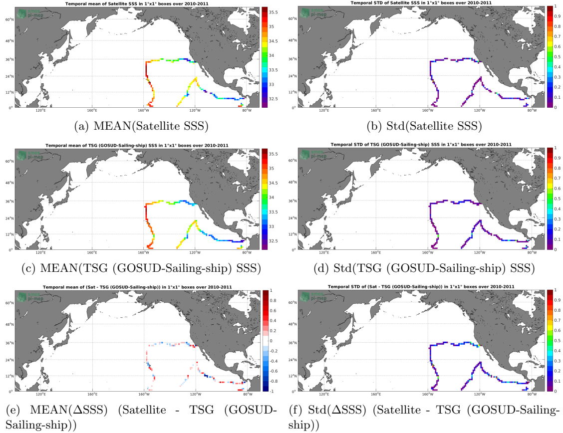
Figure 6: Temporal mean (left) and Std (right) of SSS from SMOS SSS L3 v3 Monthly (ICDC) (top), TSG (GOSUD-Sailing-ship) (middle), and of \Delta\text{SSS} (Satellite - TSG (GOSUD-Sailing-ship)). Only match-up pairs are used to generate these maps.
