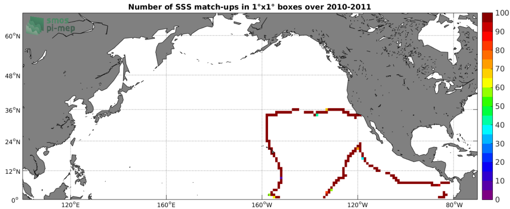
Figure 4: Number of SSS match-ups between TSG (GOSUD-Sailing-ship) SSS and the SMOS SSS L3 v3 Monthly (ICDC) SSS product for the North Pacific Ocean Pi-MEP region over 1^\circ \times 1^\circ boxes and for the full satellite product period.
