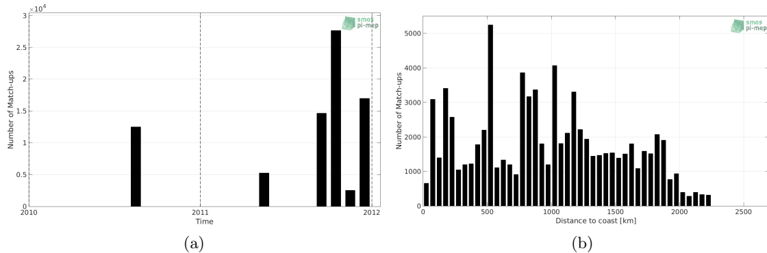
Figure 1: Number of match-ups between TSG (GOSUD-Sailing-ship) and SMOS SSS L3 v3 Monthly (ICDC) SSS as a function of time (a) and as function of the distance to coast (b) over the North Pacific Ocean Pi-MEP region and for the full satellite product period.
