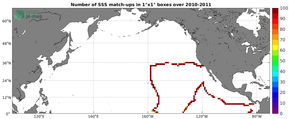
Figure 4: Number of SSS match-ups between TSG (GOSUD-Sailing-ship) SSS and the SMOS SSS L3 v3 Monthly (ICDC) SSS product for the North Pacific Ocean Pi-MEP region over 1°x1° boxes and for the full satellite product period.
