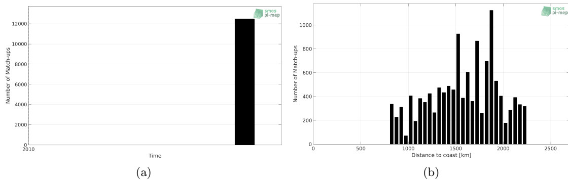
Figure 1: Number of match-ups between TSG-GOSUD-Sailing-ship and SMOS-L3-ICDC-V3-MONTHLY-0.5DEG SSS as a function of time (a) and as function of the distance to coast (b) over the North Pacific Ocean Pi-MEP region and for the full satellite product period.
