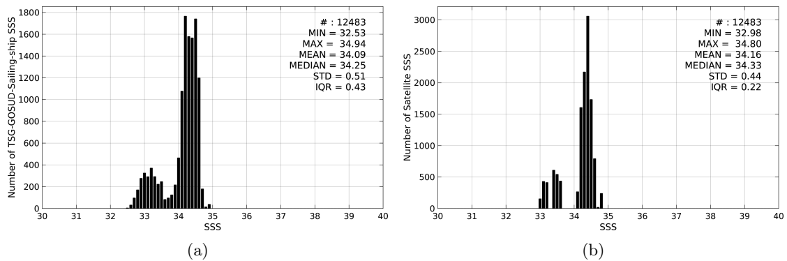
Figure 2: Histograms of SSS from TSG-GOSUD-Sailing-ship (a) and SMOS-L3-ICDC-V3-MONTHLY-0.5DEG (b) considering all match-up pairs per bins of 0.1 over the North Pacific Ocean Pi-MEP region and for the full satellite product period.
