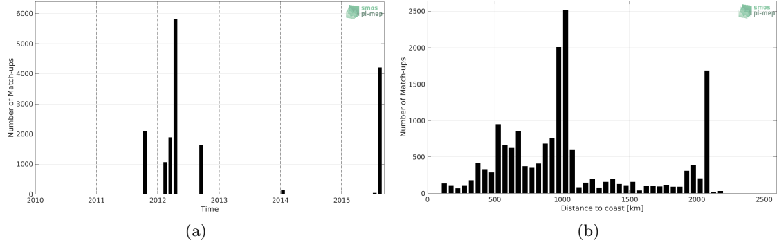
Figure 1: Number of match-ups between TSG (GOSUD-Research-vessel) and SMOS SSS L3 v3 Monthly (ICDC) SSS as a function of time (a) and as function of the distance to coast (b) over the North Pacific Ocean Pi-MEP region and for the full satellite product period.
