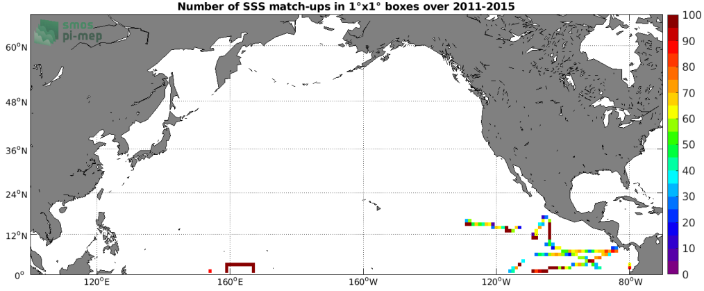
Figure 4: Number of SSS match-ups between TSG (GOSUD-Research-vessel) SSS and the SMOS SSS L3 v3 Monthly (ICDC) SSS product for the North Pacific Ocean Pi-MEP region over 1^\circ \times 1^\circ boxes and for the full satellite product period.
