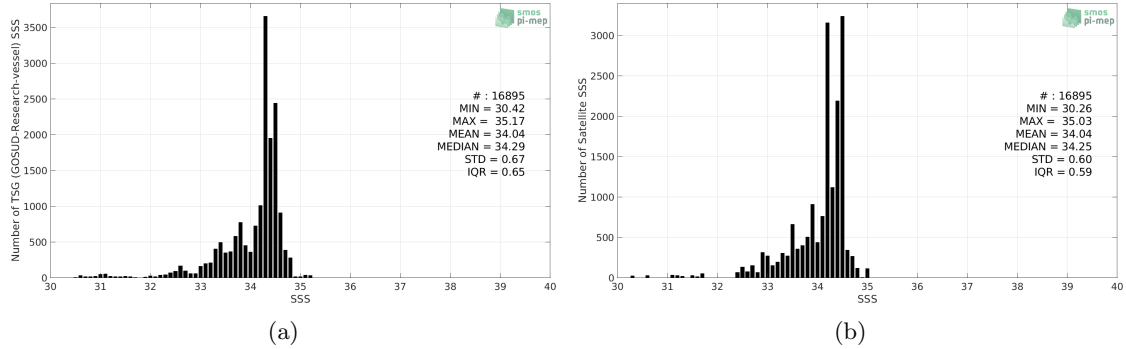
Figure 2: Histograms of SSS from TSG (GOSUD-Research-vessel) (a) and SMOS SSS L3 v3 Monthly (ICDC) (b) considering all match-up pairs per bins of 0.1 over the North Pacific Ocean Pi-MEP region and for the full satellite product period.
