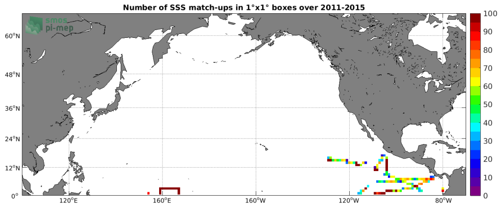
Figure 4: Number of SSS match-ups between TSG (GOSUD-Research-vessel) SSS and the SMOS SSS L3 v3 Monthly (ICDC) SSS product for the North Pacific Ocean Pi-MEP region over 1°x1° boxes and for the full satellite product period.
