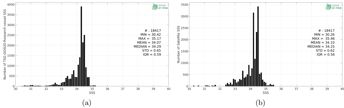
Figure 2: Histograms of SSS from TSG-GOSUD-Research-vessel (a) and SMOS-L3-ICDC-V3-MONTHLY-0.5DEG (b) considering all match-up pairs per bins of 0.1 over the North Pacific Ocean Pi-MEP region and for the full satellite product period.
