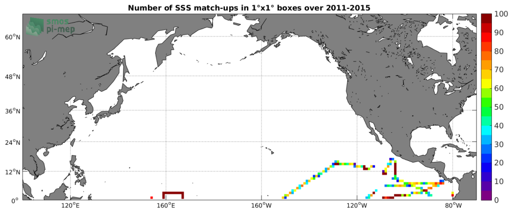
Figure 4: Number of SSS match-ups between TSG-GOSUD-Research-vessel SSS and the SMOS-L3-ICDC-V3-MONTHLY-0.5DEG SSS product for the North Pacific Ocean Pi-MEP region over 1°x1° boxes and for the full satellite product period.
