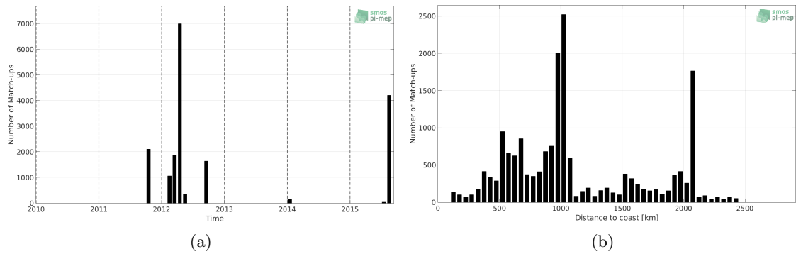
Figure 1: Number of match-ups between TSG-GOSUD-Research-vessel and SMOS-L3-ICDC-V3-MONTHLY-0.5DEG SSS as a function of time (a) and as function of the distance to coast (b) over the North Pacific Ocean Pi-MEP region and for the full satellite product period.
