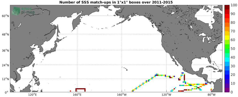
Figure 4: Number of SSS match-ups between TSG-GOSUD-Research-vessel SSS and the SMOS-L3-ICDC-V3-MONTHLY-0.5DEG SSS product for the North Pacific Ocean Pi-MEP region over 1^\circ \times 1^\circ boxes and for the full satellite product period.
