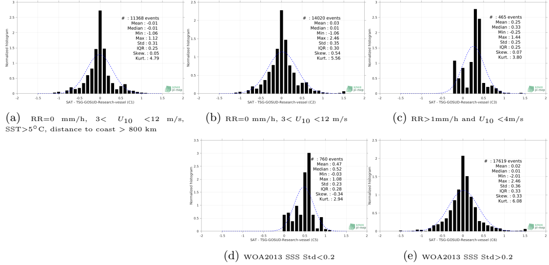
Figure 13: Normalized histogram of \Delta\text{SSS} (SMOS-L3-ICDC-V3-MONTHLY-0.5DEG - TSG-GOSUD-Research-vessel) for 5 different subdatasets corresponding to: RR=0 mm/h, 3 < U_{10} < 12 m/s, SST > 5^\circ\text{C} , distance to coast > 800 km (a), RR=0 mm/h, 3 < U_{10} < 12 m/s (b), RR > 1\text{mm/h} and U_{10} < 4\text{m/s} (c), WOA2013 SSS \text{Std} < 0.2 (d), WOA2013 SSS \text{Std} > 0.2 (e).
