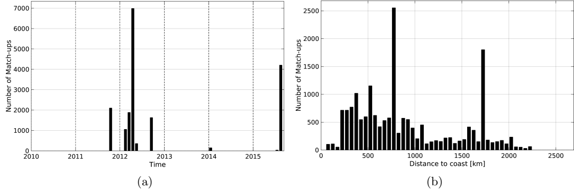
Figure 1: Number of match-ups between TSG-GOSUD-Research-vessel and SMOS-L3-ICDC-V3-MONTHLY-0.5DEG SSS as a function of time (a) and as function of the distance to coast (b) over the North Pacific Ocean Pi-MEP region and for the full satellite product period.
