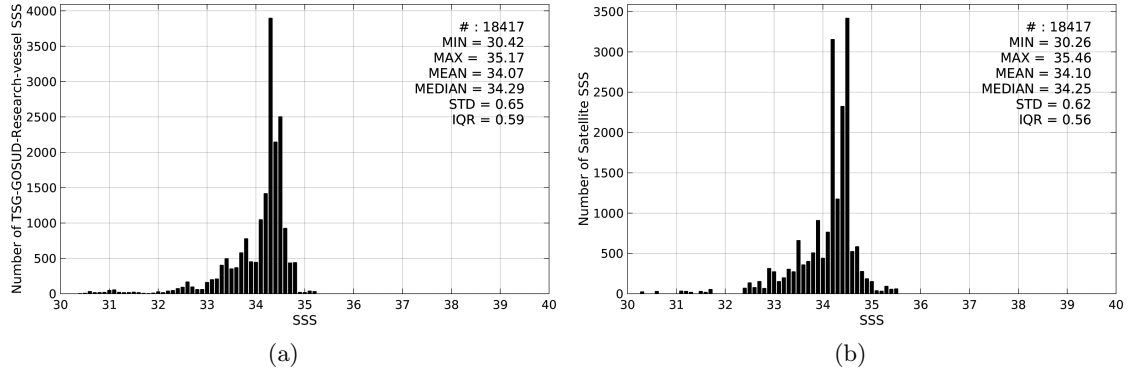
Figure 2: Histograms of SSS from TSG-GOSUD-Research-vessel (a) and SMOS-L3-ICDC-V3-MONTHLY-0.5DEG (b) considering all match-up pairs per bins of 0.1 over the North Pacific Ocean Pi-MEP region and for the full satellite product period.
