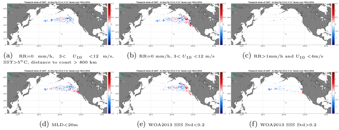
Figure 12: Temporal mean gridded over spatial boxes of size 1^\circ \times 1^\circ of \Delta SSS (SMOS SSS L3 v3 Monthly (ICDC) - Marine mammals) for 6 different subdatasets corresponding to:RR=0 mm/h, 3 < U_{10} < 12 m/s, SST >5^\circ\text{C} , distance to coast > 800 km (a), RR=0 mm/h, 3 < U_{10} < 12 m/s (b), RR >1 mm/h and U_{10} < 4 m/s (c),MLD <20 m (d),WOA2013 SSS Std <0.2 (e),WOA2013 SSS Std >0.2 (f).
