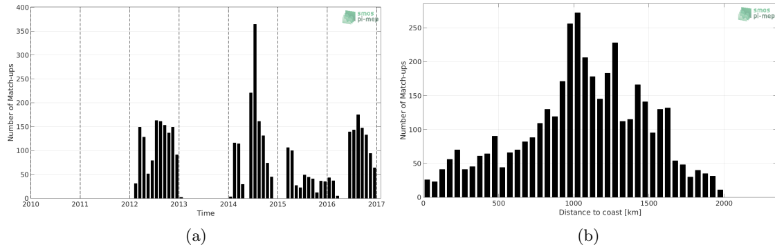
Figure 1: Number of match-ups between Marine mammals and SMOS SSS L3 v3 Monthly (ICDC) SSS as a function of time (a) and as function of the distance to coast (b) over the North Pacific Ocean Pi-MEP region and for the full satellite product period.
