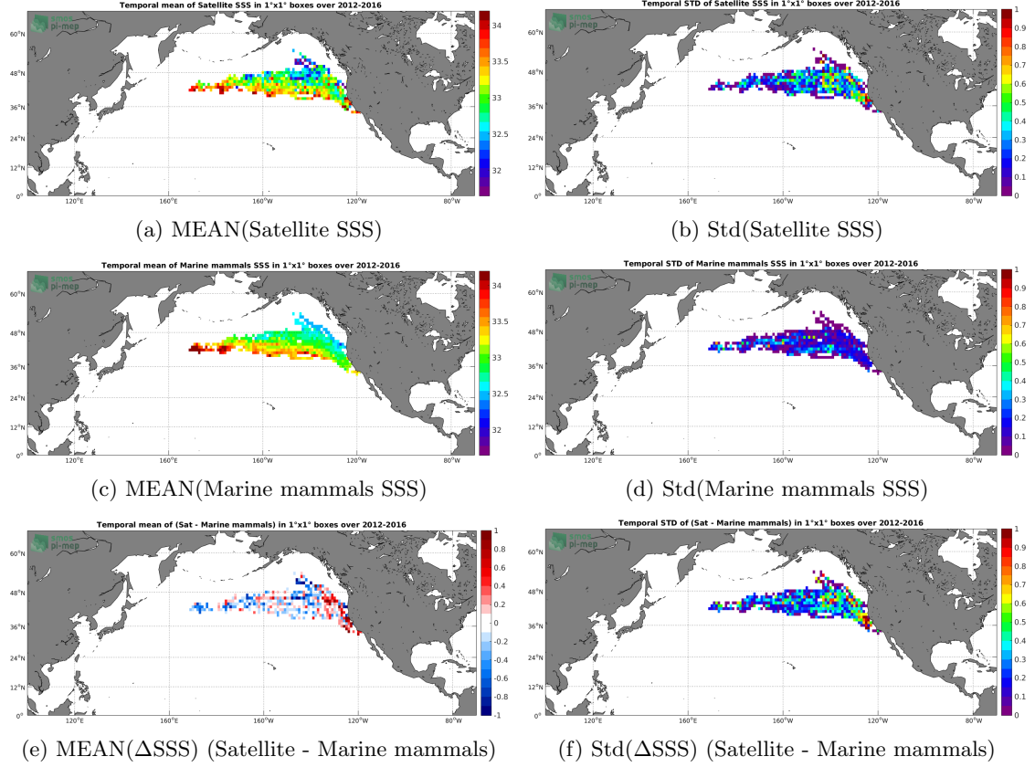
Figure 6: Temporal mean (left) and Std (right) of SSS from SMOS SSS L3 v3 Monthly (ICDC) (top), Marine mammals (middle), and of \Delta\text{SSS} (Satellite - Marine mammals). Only match-up pairs are used to generate these maps.
