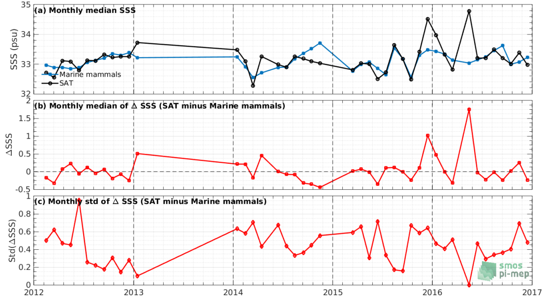
Figure 7: Time series of the monthly median SSS (top), median of \Delta\text{SSS} (Satellite - Marine mammals) and Std of \Delta\text{SSS} (Satellite - Marine mammals) over the North Pacific Ocean Pi-MEP region considering all match-ups collected by the Pi-MEP.
