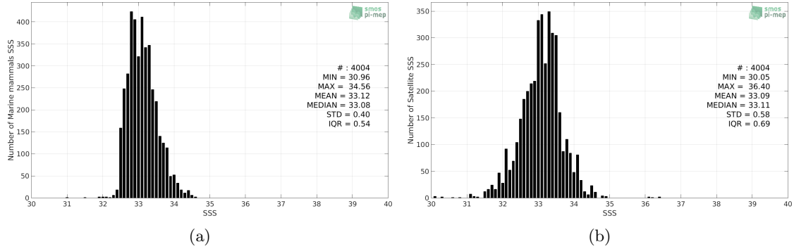
Figure 2: Histograms of SSS from Marine mammals (a) and SMOS SSS L3 v3 Monthly (ICDC) (b) considering all match-up pairs per bins of 0.1 over the North Pacific Ocean Pi-MEP region and for the full satellite product period.
