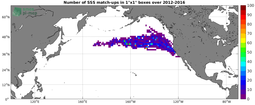
Figure 4: Number of SSS match-ups between Marine mammals SSS and the SMOS SSS L3 v3 Monthly (ICDC) SSS product for the North Pacific Ocean Pi-MEP region over 1^\circ \times 1^\circ boxes and for the full satellite product period.
