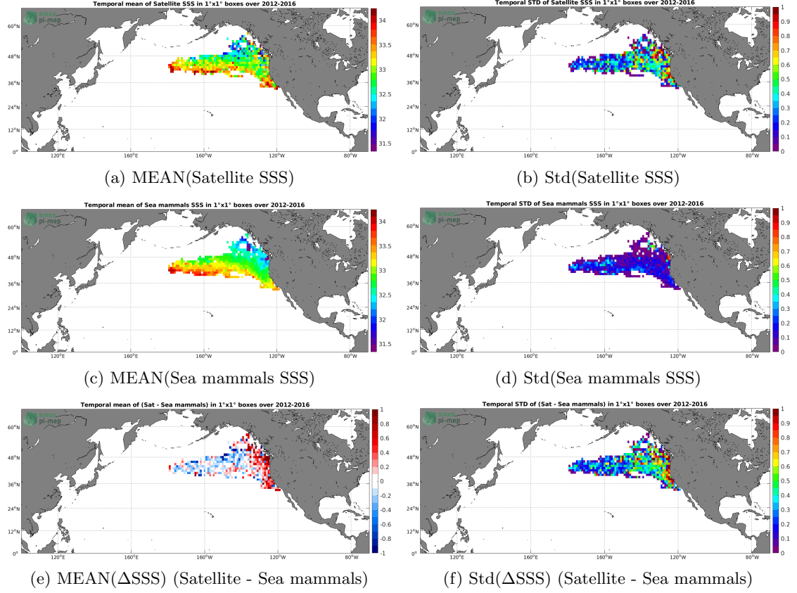
Figure 6: Temporal mean (left) and Std (right) of SSS from SMOS SSS L3 v3 Monthly (ICDC) (top), Sea mammals (middle), and of \Delta\text{SSS} (Satellite - Sea mammals). Only match-up pairs are used to generate these maps.
