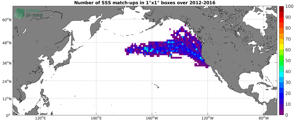
Figure 4: Number of SSS match-ups between Sea mammals SSS and the SMOS SSS L3 v3 Monthly (ICDC) SSS product for the North Pacific Ocean Pi-MEP region over 1^\circ \times 1^\circ boxes and for the full satellite product period.
