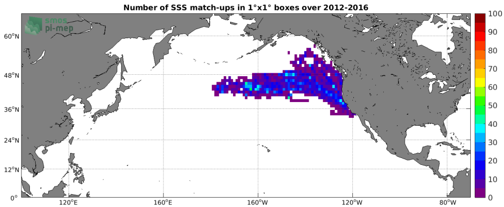
Figure 4: Number of SSS match-ups between Sea mammals SSS and the SMOS SSS L3 v3 Monthly (ICDC) SSS product for the North Pacific Ocean Pi-MEP region over 1°x1° boxes and for the full satellite product period.
