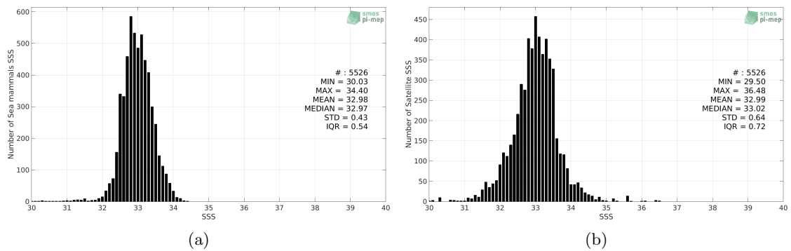
Figure 2: Histograms of SSS from Sea mammals (a) and SMOS SSS L3 v3 Monthly (ICDC) (b) considering all match-up pairs per bins of 0.1 over the North Pacific Ocean Pi-MEP region and for the full satellite product period.
