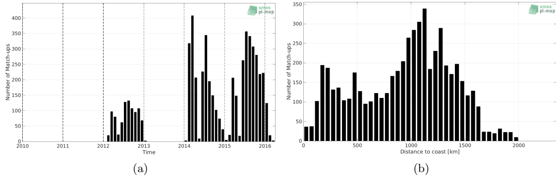
Figure 1: Number of match-ups between Sea mammals and SMOS SSS L3 v3 Monthly (ICDC) SSS as a function of time (a) and as function of the distance to coast (b) over the North Pacific Ocean Pi-MEP region and for the full satellite product period.
