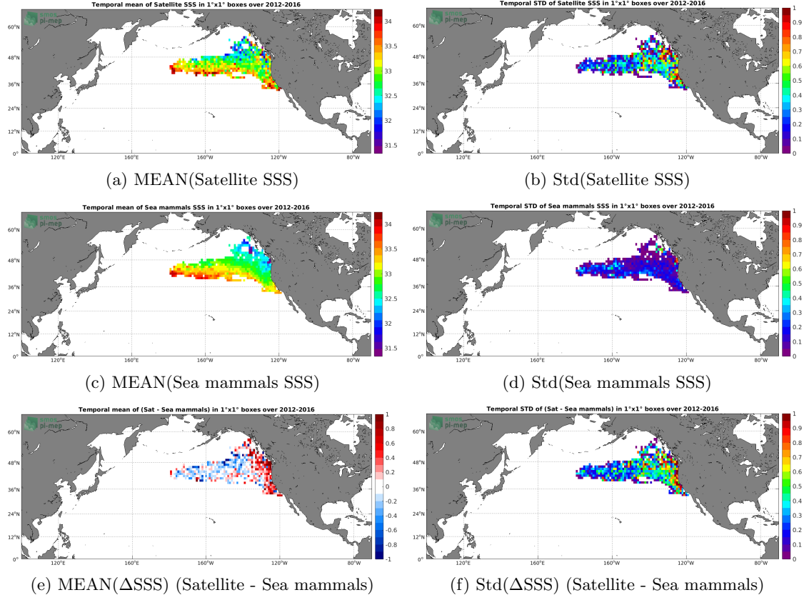
Figure 6: Temporal mean (left) and Std (right) of SSS from SMOS SSS L3 v3 Monthly (ICDC) (top), Sea mammals (middle), and of \Delta SSS (Satellite - Sea mammals). Only match-up pairs are used to generate these maps.
