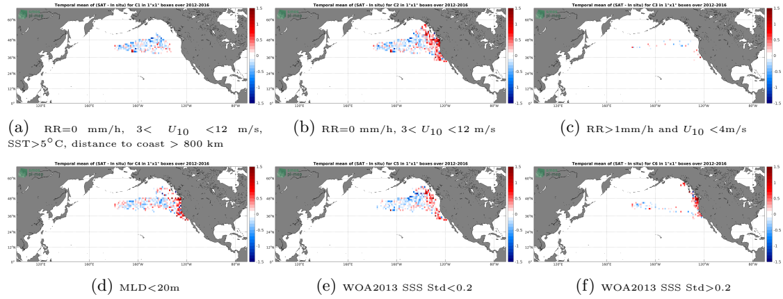
Figure 12: Temporal mean gridded over spatial boxes of size 1^\circ \times 1^\circ of \Delta SSS (SMOS SSS L3 v3 Monthly (ICDC) - Sea mammals) for 6 different subdatasets corresponding to: RR=0 mm/h, 3 < U_{10} < 12 m/s, SST > 5^\circ C , distance to coast > 800 km (a), RR=0 mm/h, 3 < U_{10} < 12 m/s (b), RR > 1 mm/h and U_{10} < 4 m/s (c), MLD < 20 m (d), WOA2013 SSS Std < 0.2 (e), WOA2013 SSS Std > 0.2 (f).
