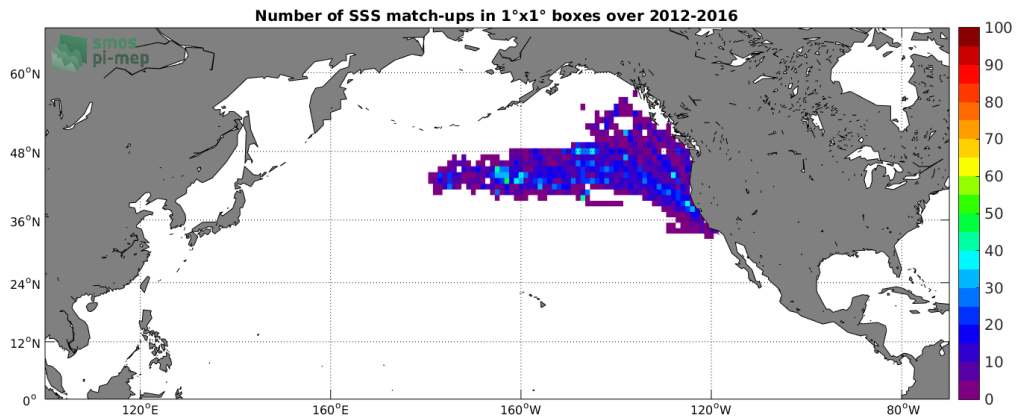
Figure 4: Number of SSS match-ups between Sea mammals SSS and the SMOS-L3-ICDC-V3-MONTHLY-0.5DEG SSS product for the North Pacific Ocean Pi-MEP region over 1°x1° boxes and for the full satellite product period.
