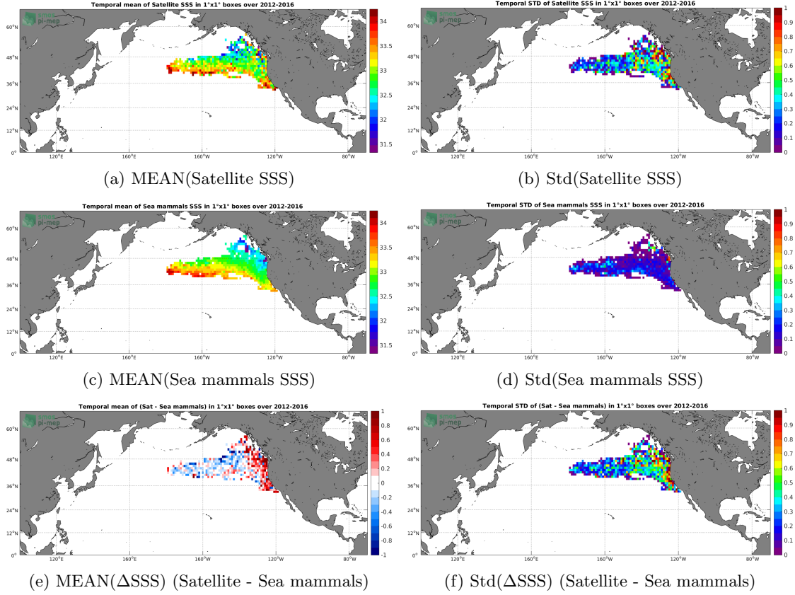
Figure 6: Temporal mean (left) and Std (right) of SSS from SMOS-L3-ICDC-V3-MONTHLY-0.5DEG (top), Sea mammals (middle), and of \Delta SSS (Satellite - Sea mammals). Only match-up pairs are used to generate these maps.
