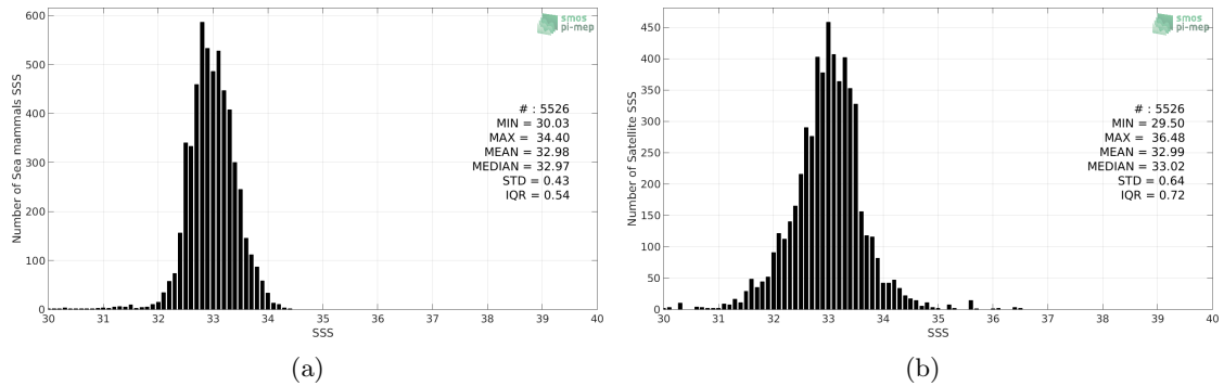
Figure 2: Histograms of SSS from Sea mammals (a) and SMOS-L3-ICDC-V3-MONTHLY-0.5DEG (b) considering all match-up pairs per bins of 0.1 over the North Pacific Ocean Pi-MEP region and for the full satellite product period.
