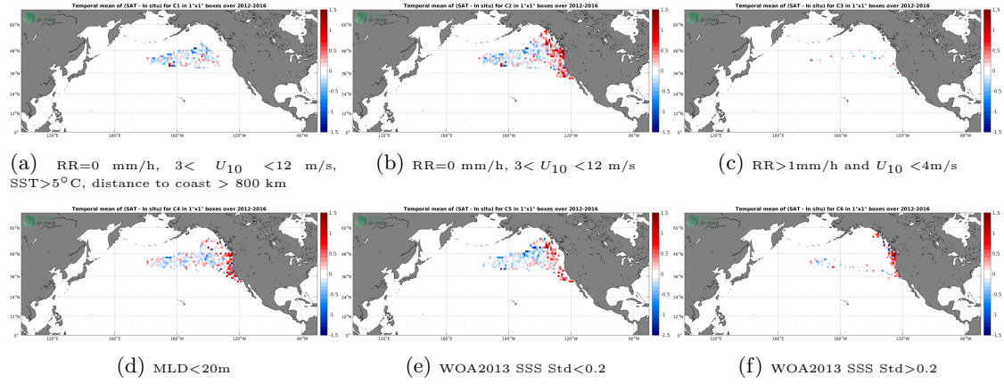
Figure 12: Temporal mean gridded over spatial boxes of size 1^\circ \times 1^\circ of \Delta SSS (SMOS-L3-ICDC-V3-MONTHLY-0.5DEG - Sea mammals) for 6 different subdatasets corresponding to: RR=0 mm/h, 3 < U_{10} < 12 m/s, SST > 5^\circ\text{C} , distance to coast > 800 km (a), RR=0 mm/h, 3 < U_{10} < 12 m/s (b), RR > 1 mm/h and U_{10} < 4 m/s (c), MLD < 20 m (d), WOA2013 SSS Std < 0.2 (e), WOA2013 SSS Std > 0.2 (f).
