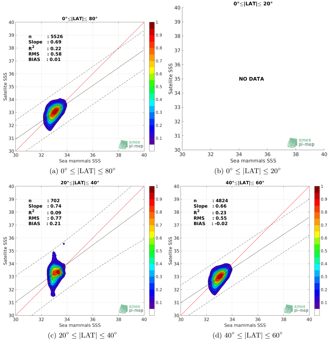
Figure 9: Contour maps of the concentration of SMOS-L3-ICDC-V3-MONTHLY-0.5DEG SSS (y-axis) versus Sea mammals SSS (x-axis) at match-up pairs for different latitude bands. For each plot, the red line shows x=y . The black thin and dashed lines indicate a linear fit through the data cloud and the \pm 95\% confidence levels, respectively. The number match-up pairs n , the slope and R^2 coefficient of the linear fit, the root mean square (RMS) and the mean bias between satellite and in situ data are indicated for each latitude band in each plots.
