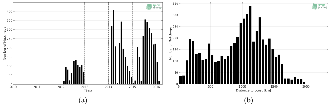
Figure 1: Number of match-ups between Sea mammals and SMOS-L3-ICDC-V3-MONTHLY-0.5DEG SSS as a function of time (a) and as function of the distance to coast (b) over the North Pacific Ocean Pi-MEP region and for the full satellite product period.
