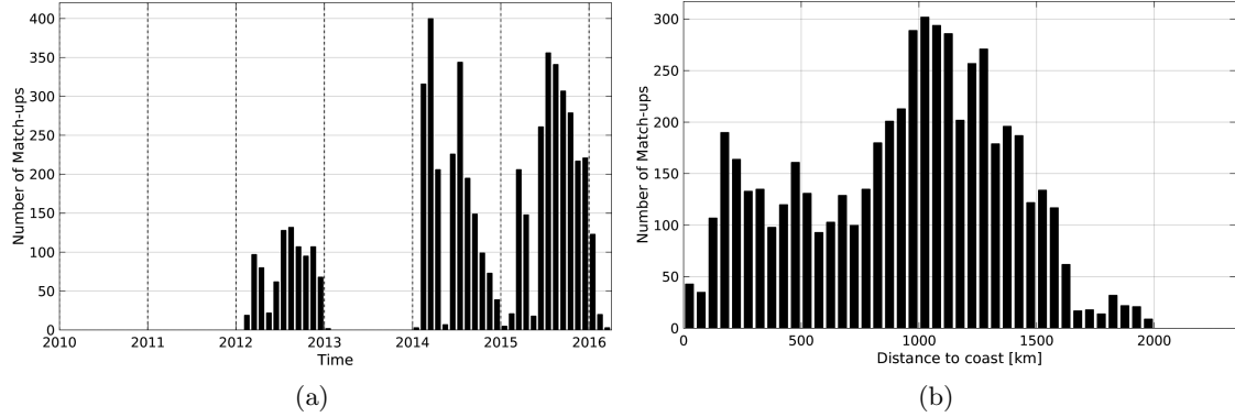
Figure 1: Number of match-ups between Sea mammals and SMOS-L3-ICDC-V3-MONTHLY-0.5DEG SSS as a function of time (a) and as function of the distance to coast (b) over the North Pacific Ocean Pi-MEP region and for the full satellite product period.
