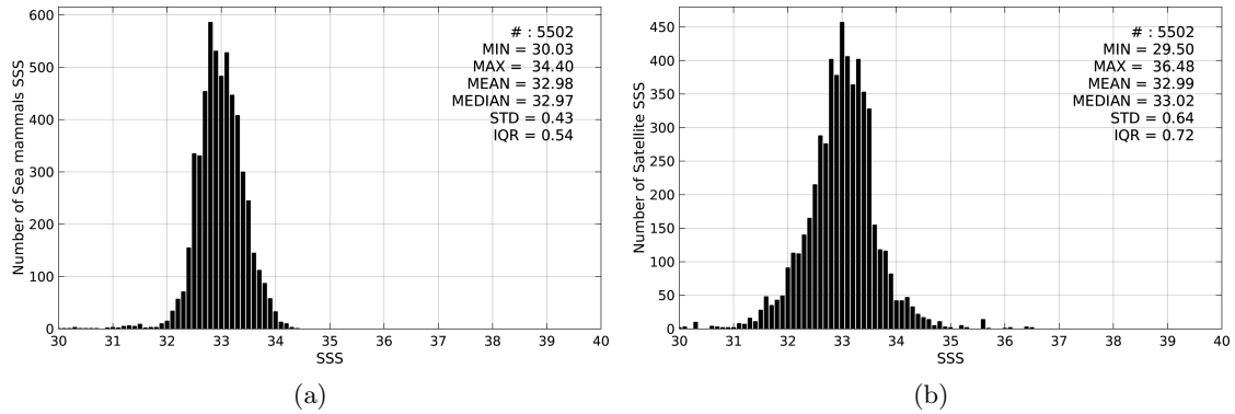
Figure 2: Histograms of SSS from Sea mammals (a) and SMOS-L3-ICDC-V3-MONTHLY-0.5DEG (b) considering all match-up pairs per bins of 0.1 over the North Pacific Ocean Pi-MEP region and for the full satellite product period.
