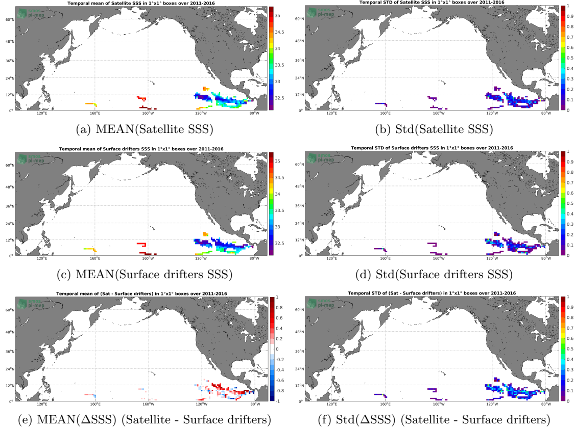
Figure 5: Temporal mean (left) and Std (right) of SSS from SMOS SSS L3 v3 Monthly (ICDC) (top), Surface drifters (middle), and of \Delta SSS (Satellite - Surface drifters). Only match-up pairs are used to generate these maps.
