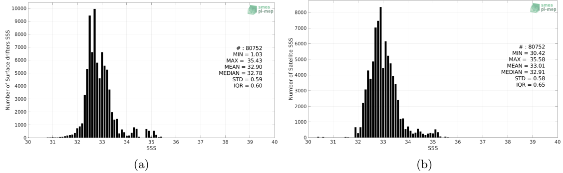
Figure 2: Histograms of SSS from Surface drifters (a) and SMOS SSS L3 v3 Monthly (ICDC) (b) considering all match-up pairs per bins of 0.1 over the North Pacific Ocean Pi-MEP region and for the full satellite product period.
