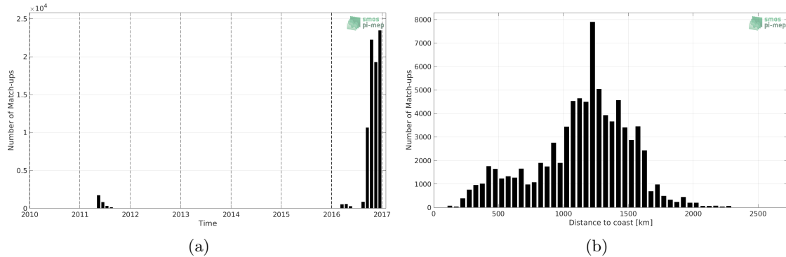
Figure 1: Number of match-ups between Surface drifters and SMOS SSS L3 v3 Monthly (ICDC) SSS as a function of time (a) and as function of the distance to coast (b) over the North Pacific Ocean Pi-MEP region and for the full satellite product period.
