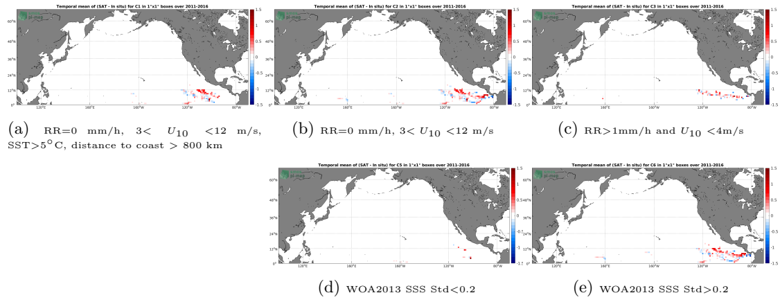
Figure 11: Temporal mean gridded over spatial boxes of size 1^\circ \times 1^\circ of \Delta SSS (SMOS SSS L3 v3 Monthly (ICDC) - Surface drifters) for 5 different subdatasets corresponding to: RR=0 mm/h, 3 < U_{10} < 12 m/s, SST > 5^\circ C , distance to coast > 800 km (a), RR=0 mm/h, 3 < U_{10} < 12 m/s (b), RR > 1 mm/h and U_{10} < 4 m/s (c), WOA2013 SSS Std < 0.2 (d), WOA2013 SSS Std > 0.2 (e).
