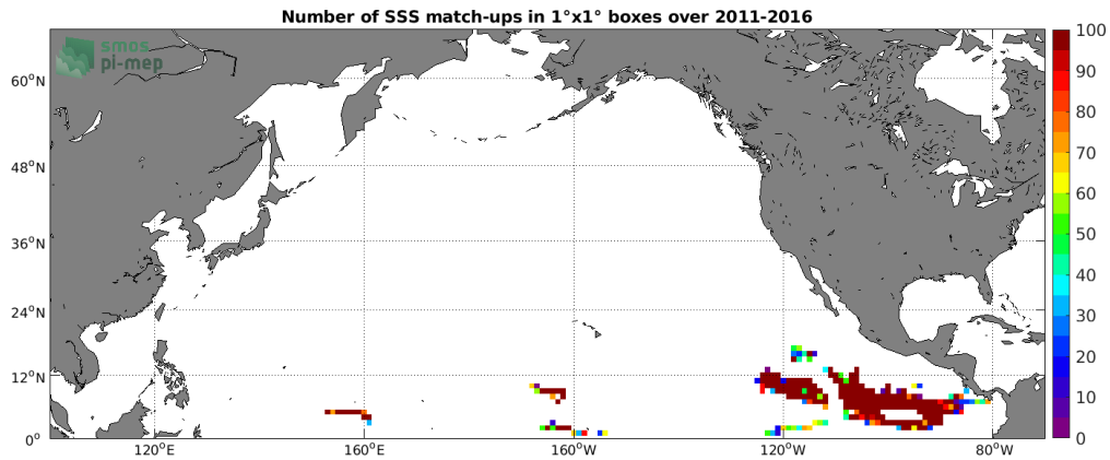
Figure 3: Number of SSS match-ups between Surface drifters SSS and the SMOS SSS L3 v3 Monthly (ICDC) SSS product for the North Pacific Ocean Pi-MEP region over 1^\circ \times 1^\circ boxes and for the full satellite product period.
