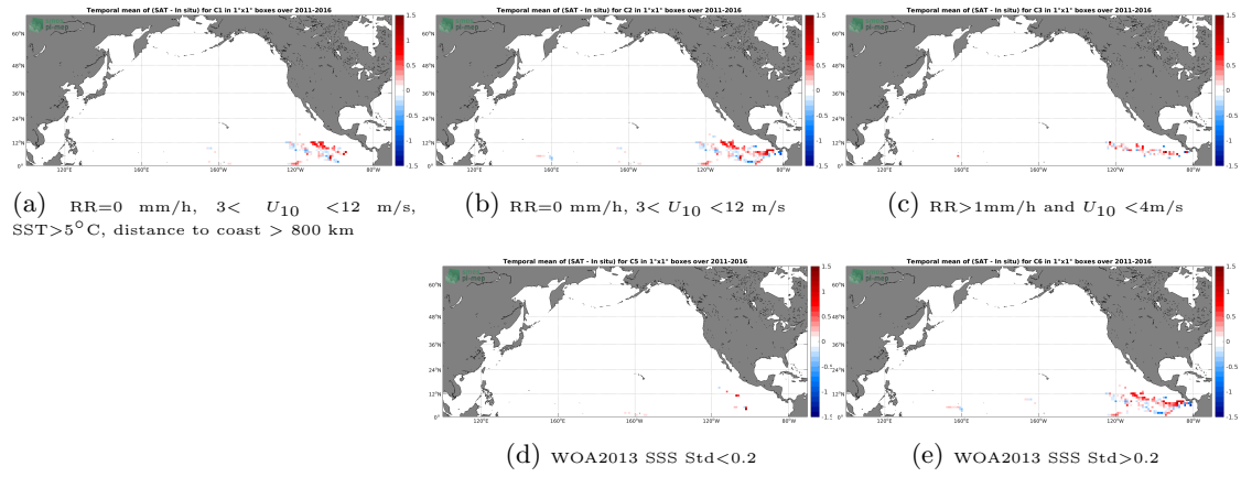
Figure 11: Temporal mean gridded over spatial boxes of size 1^\circ \times 1^\circ of \Delta SSS (SMOS SSS L3 v3 Monthly (ICDC) - Surface drifters) for 5 different subdatasets corresponding to:RR=0 mm/h, 3 < U_{10} < 12 m/s, SST >5^\circ\text{C} , distance to coast > 800 km (a), RR=0 mm/h, 3 < U_{10} < 12 m/s (b), RR >1 mm/h and U_{10} < 4 m/s (c), WOA2013 SSS Std <0.2 (d), WOA2013 SSS Std >0.2 (e).
