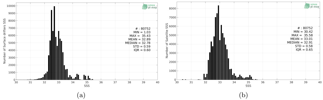
Figure 2: Histograms of SSS from Surface drifters (a) and SMOS SSS L3 v3 Monthly (ICDC) (b) considering all match-up pairs per bins of 0.1 over the North Pacific Ocean Pi-MEP region and for the full satellite product period.
