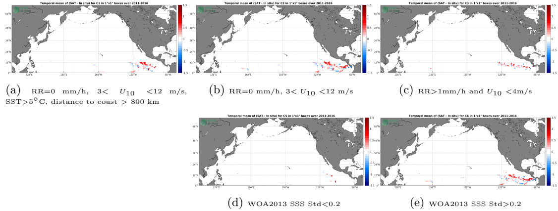
Figure 11: Temporal mean gridded over spatial boxes of size 1^\circ \times 1^\circ of \Delta SSS (SMOS-L3-ICDC-V3-MONTHLY-0.5DEG - Surface drifters) for 5 different subdatasets corresponding to: RR=0 mm/h, 3 < U_{10} < 12 m/s, SST >5^\circ\text{C} , distance to coast > 800 km (a), RR=0 mm/h, 3 < U_{10} < 12 m/s (b), RR >1 mm/h and U_{10} < 4 m/s (c), WOA2013 SSS Std <0.2 (d), WOA2013 SSS Std >0.2 (e).
