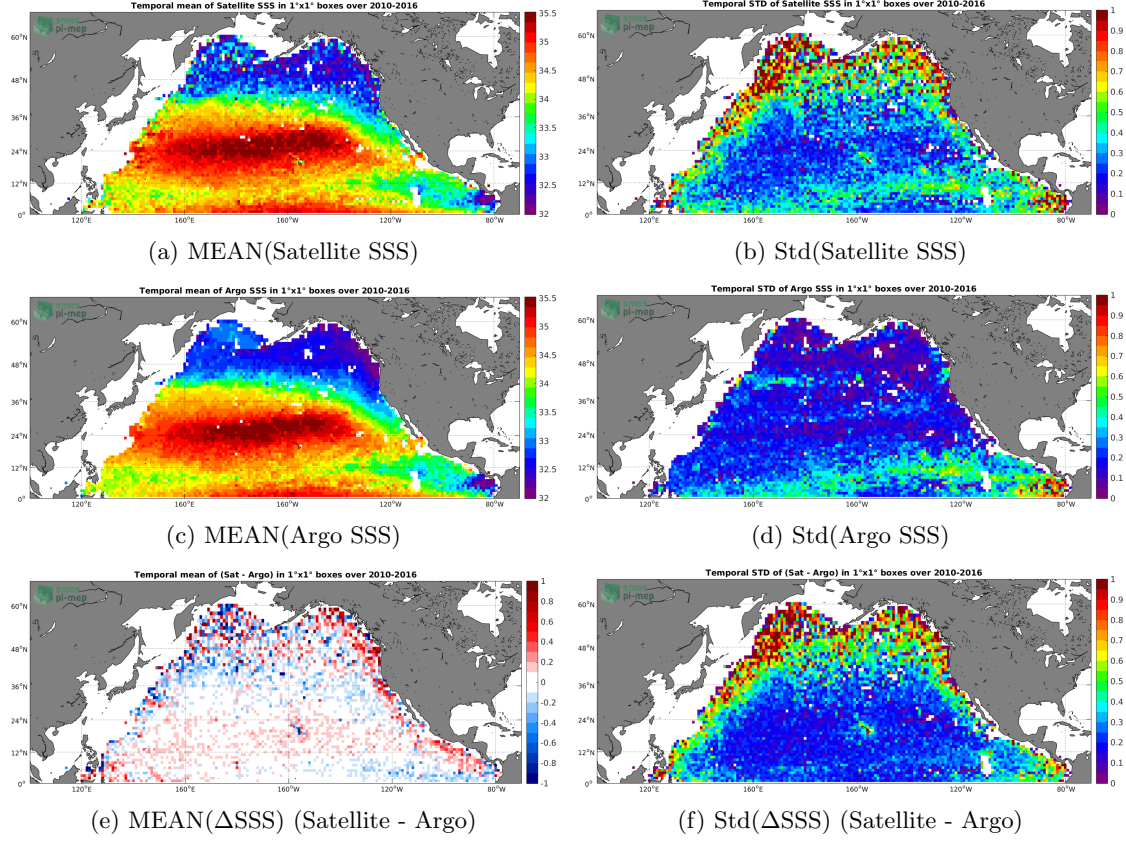
Figure 6: Temporal mean (left) and Std (right) of SSS from SMOS SSS L3 v3 Monthly (ICDC) (top), Argo (middle), and of \Delta\text{SSS} (Satellite - Argo). Only match-up pairs are used to generate these maps.
