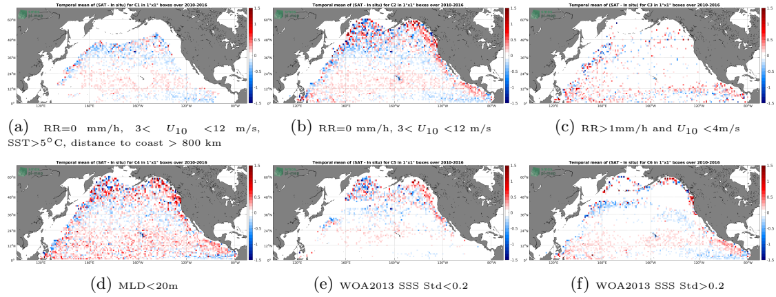
Figure 12: Temporal mean gridded over spatial boxes of size 1^\circ \times 1^\circ of \Delta SSS (SMOS SSS L3 v3 Monthly (ICDC) - Argo) for 6 different subdatasets corresponding to: RR=0 mm/h, 3 < U_{10} < 12 m/s, SST > 5^\circ\text{C} , distance to coast > 800 km (a), RR=0 mm/h, 3 < U_{10} < 12 m/s (b), RR > 1 mm/h and U_{10} < 4 m/s (c), MLD < 20 m (d), WOA2013 SSS Std < 0.2 (e), WOA2013 SSS Std > 0.2 (f).
