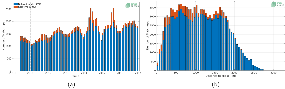
Figure 1: Number of match-ups between Argo and SMOS SSS L3 v3 Monthly (ICDC) SSS as a function of time (a) and as function of the distance to coast (b) over the North Pacific Ocean Pi-MEP region and for the full satellite product period.
