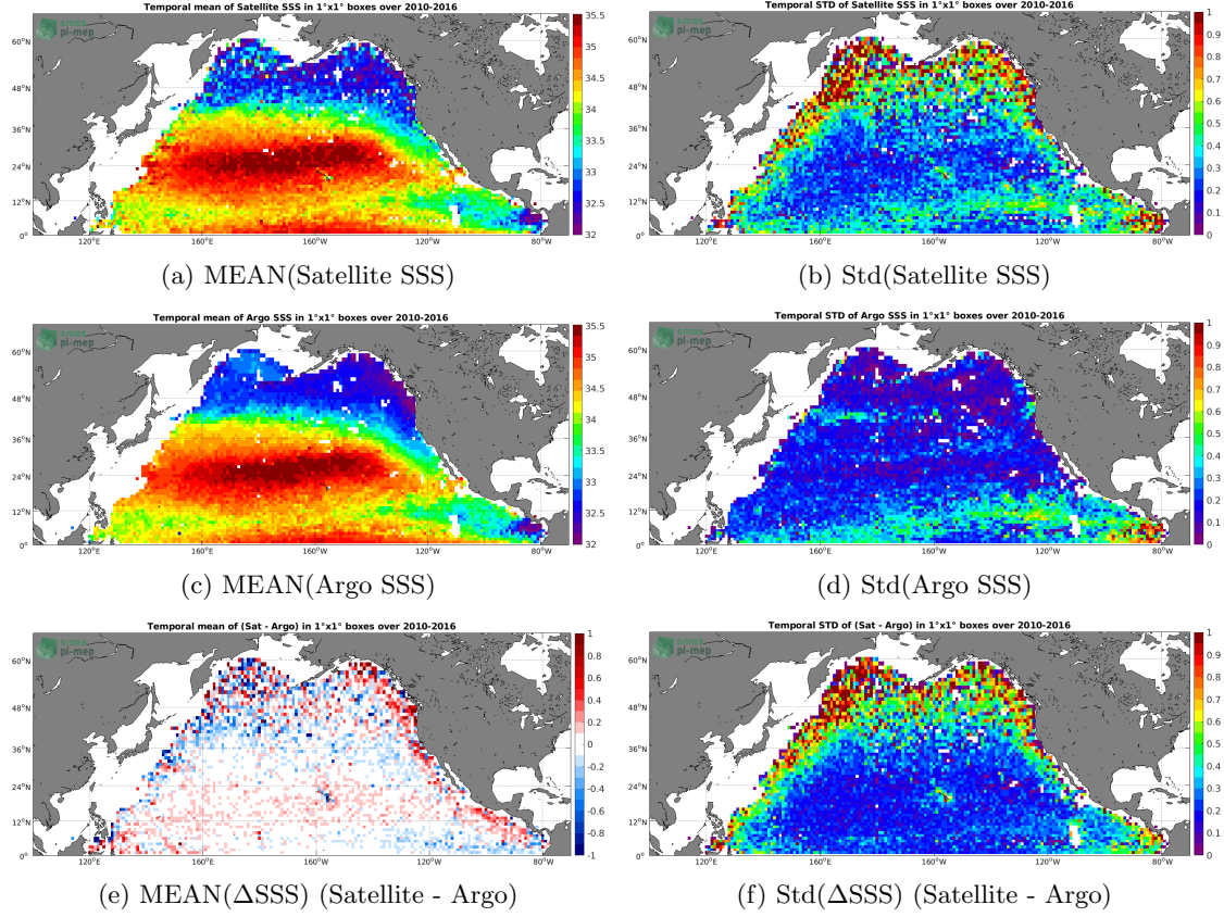
Figure 6: Temporal mean (left) and Std (right) of SSS from SMOS SSS L3 v3 Monthly (ICDC) (top), Argo (middle), and of \Delta SSS (Satellite - Argo). Only match-up pairs are used to generate these maps.
