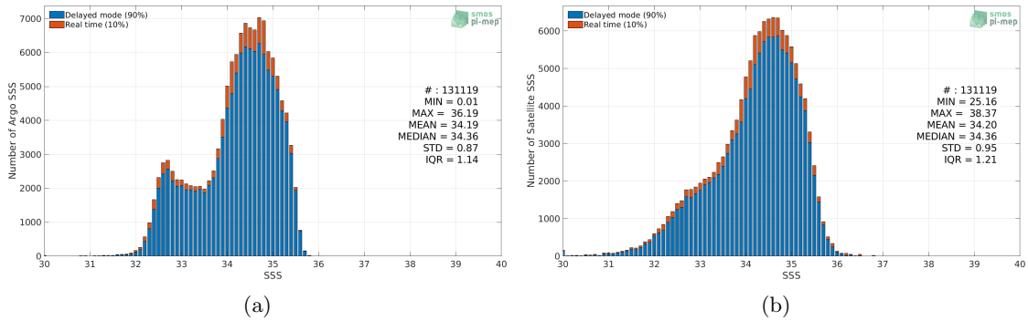
Figure 2: Histograms of SSS from Argo (a) and SMOS SSS L3 v3 Monthly (ICDC) (b) considering all match-up pairs per bins of 0.1 over the North Pacific Ocean Pi-MEP region and for the full satellite product period.
