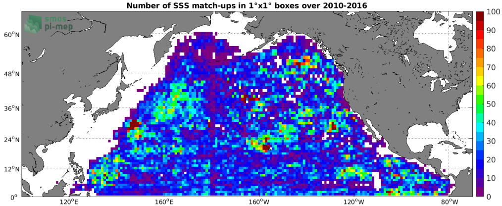
Figure 4: Number of SSS match-ups between Argo SSS and the SMOS SSS L3 v3 Monthly (ICDC) SSS product for the North Pacific Ocean Pi-MEP region over 1^\circ \times 1^\circ boxes and for the full satellite product period.
