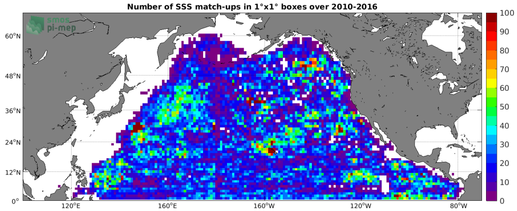
Figure 4: Number of SSS match-ups between Argo SSS and the SMOS SSS L3 v3 Monthly (ICDC) SSS product for the North Pacific Ocean Pi-MEP region over 1°x1° boxes and for the full satellite product period.
