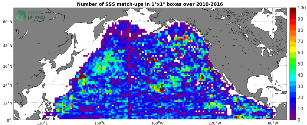
Figure 4: Number of SSS match-ups between Argos SSS and the SMOS-L3-ICDC-V3-MONTHLY-0.5DEG SSS product for the North Pacific Ocean Pi-MEP region over 1^\circ \times 1^\circ boxes and for the full satellite product period.
