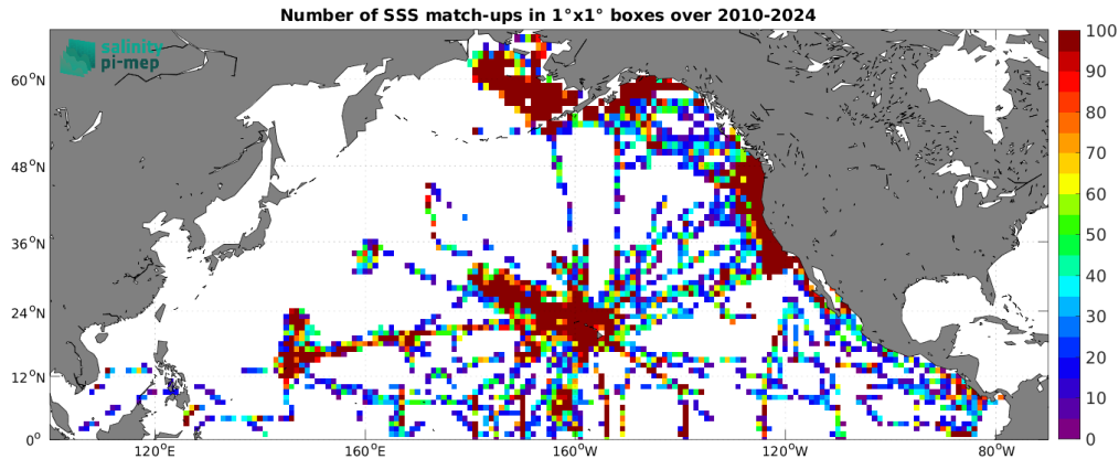
Figure 5: Number of SSS match-ups between TSG (SAMOS) SSS and the SMOS SSS L2Q v331 - With FLAG (CMEMS-CATDS-CPDC) SSS product for the North Pacific Ocean Pi-MEP region over 1^\circ \times 1^\circ boxes and for the full satellite product period.
