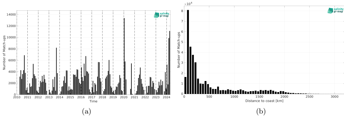
Figure 2: Number of match-ups between TSG (SAMOS) and SMOS SSS L2Q v331 - With FLAG (CMEMS-CATDS-CPDC) SSS as a function of time (a) and as function of the distance to coast (b) over the North Pacific Ocean Pi-MEP region and for the full satellite product period.
