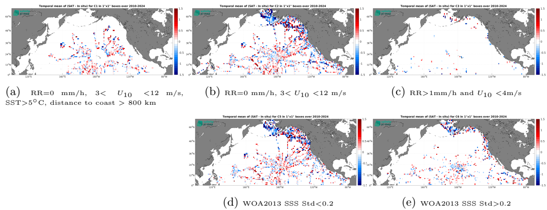
Figure 14: Temporal mean gridded over spatial boxes of size 1^\circ \times 1^\circ of \Delta\text{SSS} (SMOS SSS L2Q v331 - With FLAG (CMEMS-CATDS-CPDC) - TSG (SAMOS)) for 5 different subdatasets corresponding to:RR=0 mm/h, 3 < U_{10} < 12 m/s, SST>5°C, distance to coast > 800 km (a), RR=0 mm/h, 3 < U_{10} < 12 m/s (b), RR>1mm/h and U_{10} < 4 m/s (c), WOA2013 SSS Std<0.2 (d), WOA2013 SSS Std>0.2 (e).
