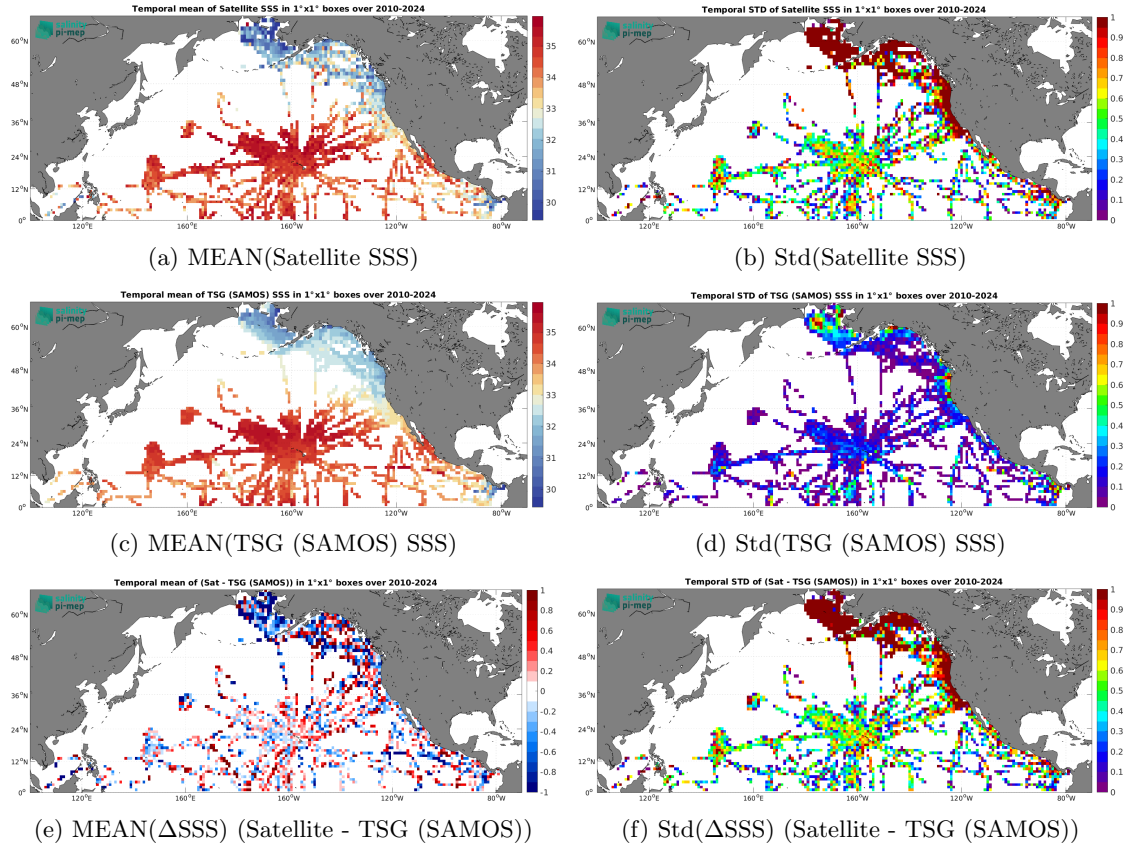
Figure 7: Temporal mean (left) and Std (right) of SSS from SMOS SSS L2Q v331 - With FLAG (CMEMS-CATDS-CPDC) (top), TSG (SAMOS) (middle), and of \Delta SSS (Satellite - TSG (SAMOS)). Only match-up pairs are used to generate these maps.
