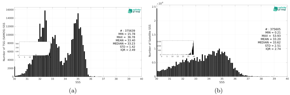
Figure 3: Histograms of SSS from TSG (SAMOS) (a) and SMOS SSS L2Q v331 - With FLAG (CMEMS-CATDS-CPDC) (b) considering all match-up pairs per bins of 0.1 over the North Pacific Ocean Pi-MEP region and for the full satellite product period.
