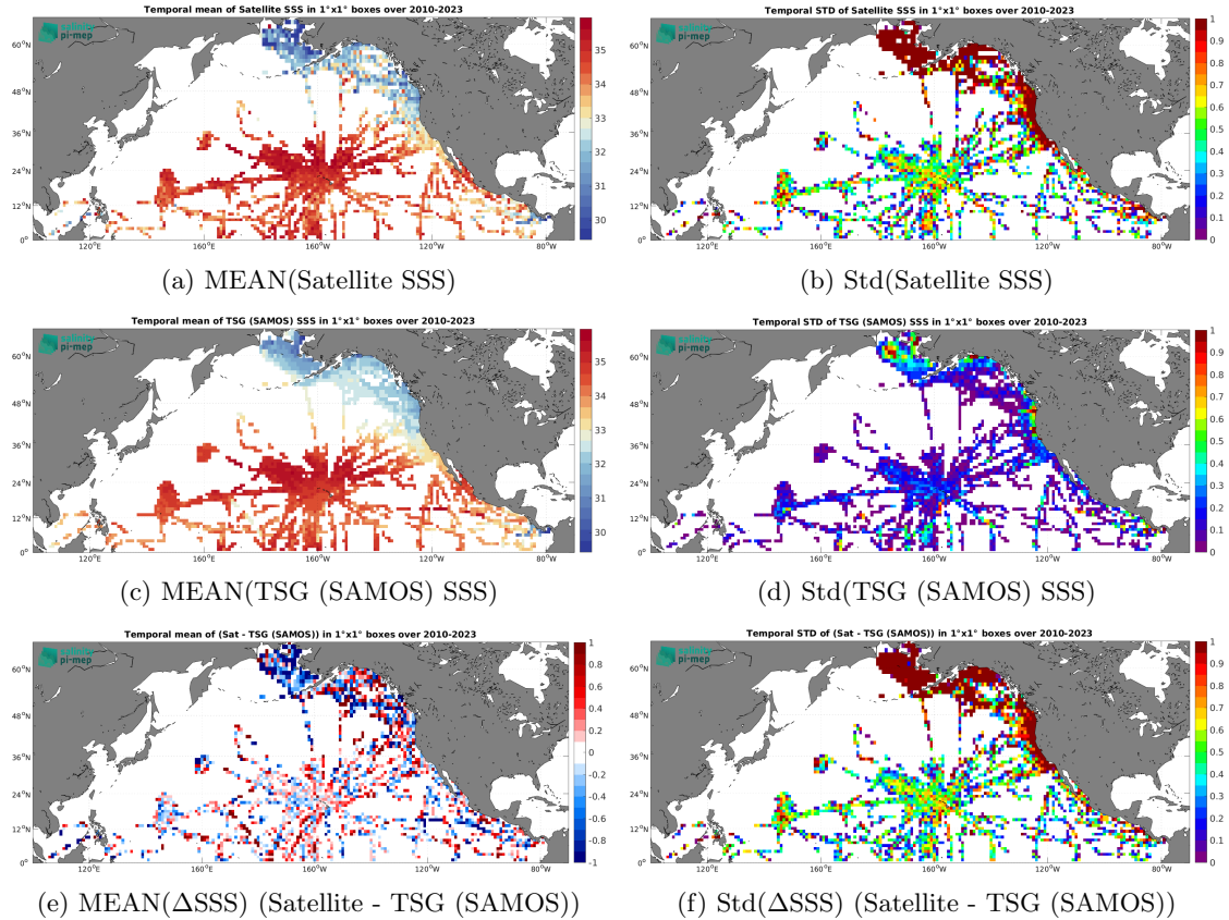
Figure 6: Temporal mean (left) and Std (right) of SSS from SMOS SSS L2Q v331 - With FLAG (CMEMS-CATDS-CPDC) (top), TSG (SAMOS) (middle), and of \Delta SSS (Satellite - TSG (SAMOS)). Only match-up pairs are used to generate these maps.
