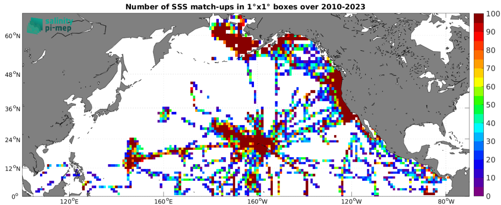
Figure 4: Number of SSS match-ups between TSG (SAMOS) SSS and the SMOS SSS L2Q v331 - With FLAG (CMEMS-CATDS-CPDC) SSS product for the North Pacific Ocean Pi-MEP region over 1^\circ \times 1^\circ boxes and for the full satellite product period.
