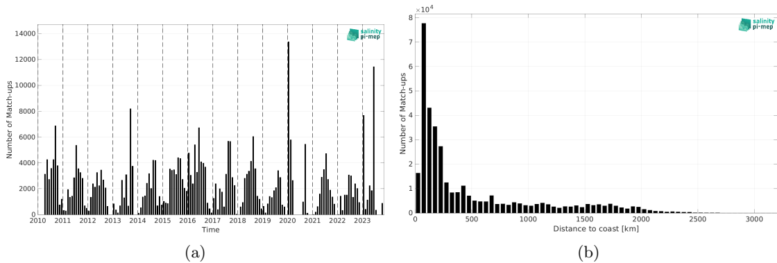
Figure 1: Number of match-ups between TSG (SAMOS) and SMOS SSS L2Q v331 - With FLAG (CMEMS-CATDS-CPDC) SSS as a function of time (a) and as function of the distance to coast (b) over the North Pacific Ocean Pi-MEP region and for the full satellite product period.
