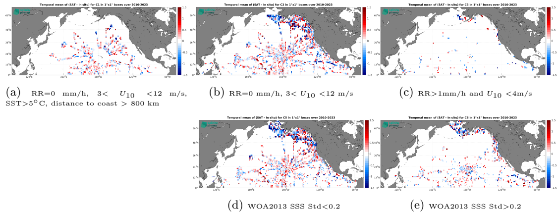
Figure 12: Temporal mean gridded over spatial boxes of size 1^\circ \times 1^\circ of \Delta SSS (SMOS SSS L2Q v331 - With FLAG (CMEMS-CATDS-CPDC) - TSG (SAMOS)) for 5 different subdatasets corresponding to:RR=0 mm/h, 3 < U_{10} < 12 m/s, SST >5^\circ C, distance to coast > 800 km (a), RR=0 mm/h, 3 < U_{10} < 12 m/s (b), RR >1 mm/h and U_{10} < 4 m/s (c), WOA2013 SSS Std <0.2 (d), WOA2013 SSS Std >0.2 (e).
