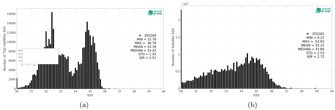
Figure 2: Histograms of SSS from TSG (SAMOS) (a) and SMOS SSS L2Q v331 - With FLAG (CMEMS-CATDS-CPDC) (b) considering all match-up pairs per bins of 0.1 over the North Pacific Ocean Pi-MEP region and for the full satellite product period.
