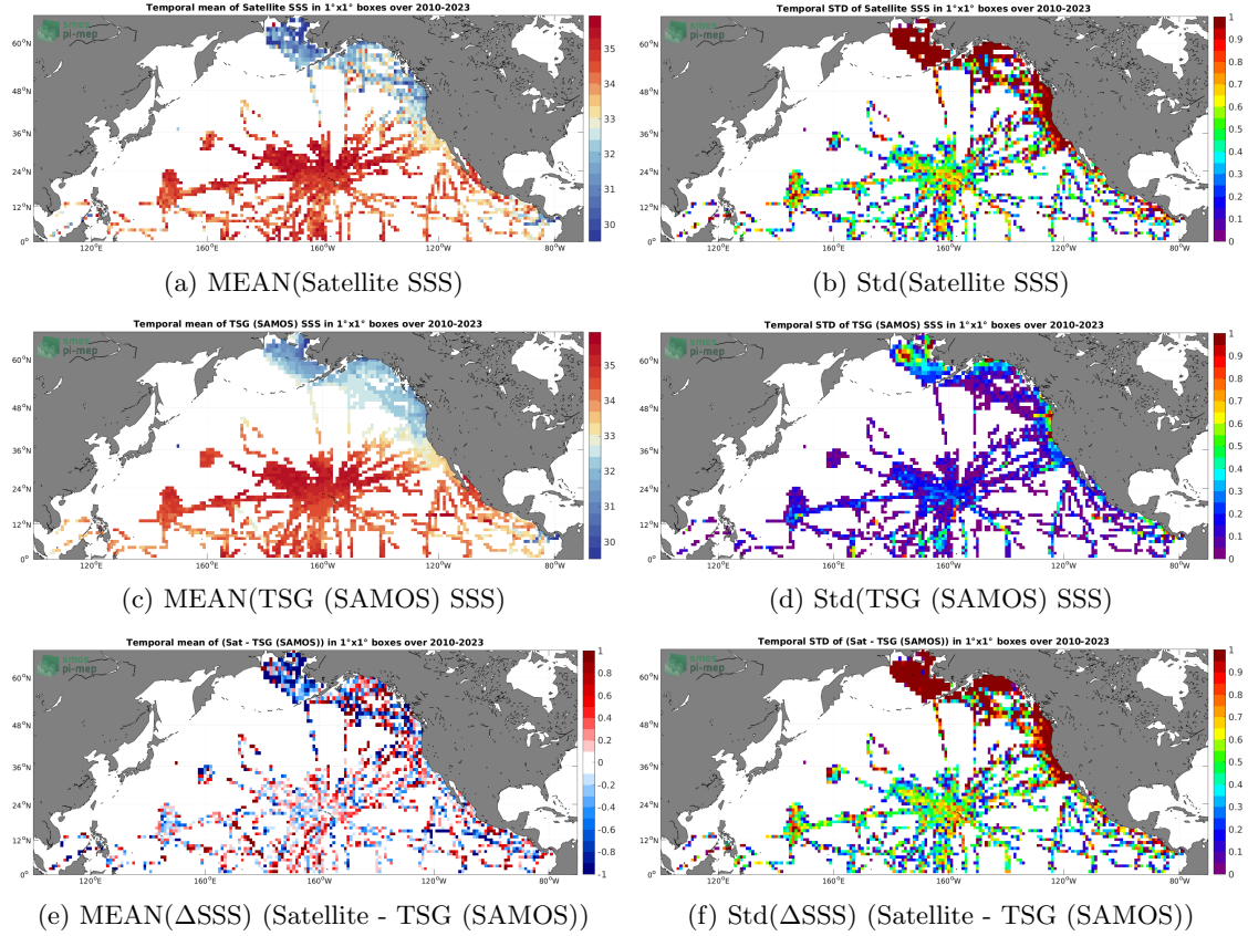
Figure 6: Temporal mean (left) and Std (right) of SSS from SMOS SSS L2Q v331 - With FLAG (CMEMS-CATDS-CPDC) (top), TSG (SAMOS) (middle), and of \Delta\text{SSS} (Satellite - TSG (SAMOS)). Only match-up pairs are used to generate these maps.
