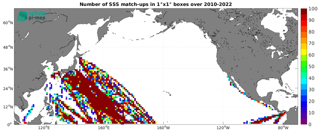
Figure 5: Number of SSS match-ups between TSG (LEGOS-DM) SSS and the SMOS SSS L2Q v331 - With FLAG (CMEMS-CATDS-CPDC) SSS product for the North Pacific Ocean Pi-MEP region over 1^\circ \times 1^\circ boxes and for the full satellite product period.
