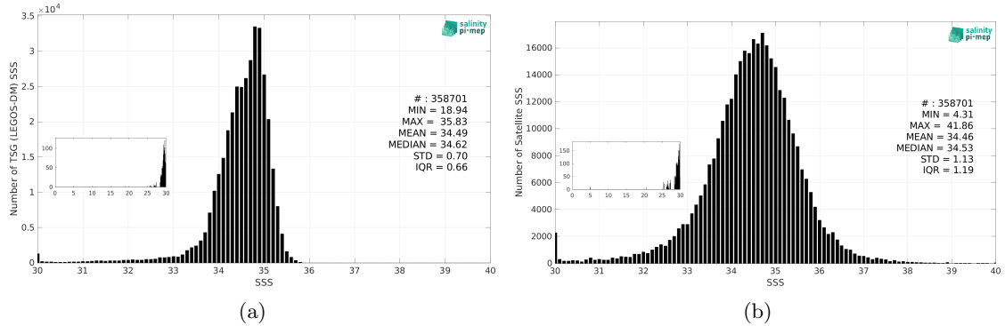
Figure 3: Histograms of SSS from TSG (LEGOS-DM) (a) and SMOS SSS L2Q v331 - With FLAG (CMEMS-CATDS-CPDC) (b) considering all match-up pairs per bins of 0.1 over the North Pacific Ocean Pi-MEP region and for the full satellite product period.
