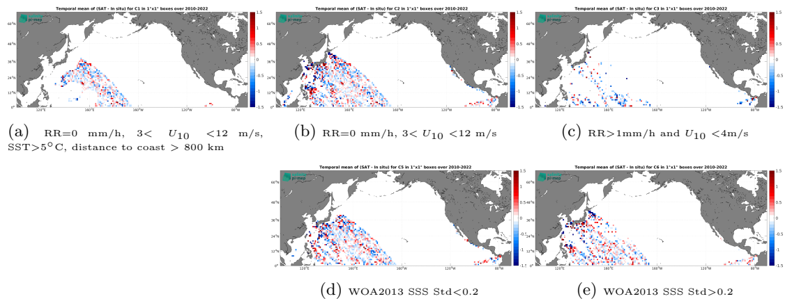
Figure 14: Temporal mean gridded over spatial boxes of size 1^\circ \times 1^\circ of \Delta\text{SSS} (SMOS SSS L2Q v331 - With FLAG (CMEMS-CATDS-CPDC) - TSG (LEGOS-DM)) for 5 different subdatasets corresponding to: RR=0 mm/h, 3 < U_{10} < 12 m/s, SST > 5°C, distance to coast > 800 km (a), RR=0 mm/h, 3 < U_{10} < 12 m/s (b), RR > 1 mm/h and U_{10} < 4 m/s (c), WOA2013 SSS Std < 0.2 (d), WOA2013 SSS Std > 0.2 (e).
