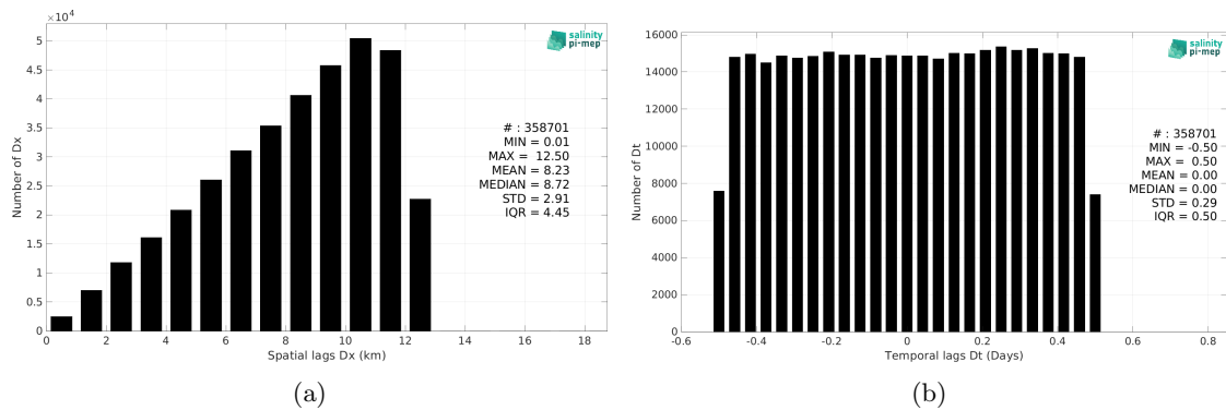
Figure 6: Histograms of the spatial (a) and temporal (b) lags between the location/time of the TSG (LEGOS-DM) measurement and the date of the corresponding SMOS SSS L2Q v331 - With FLAG (CMEMS-CATDS-CPDC) SSS pixel.
