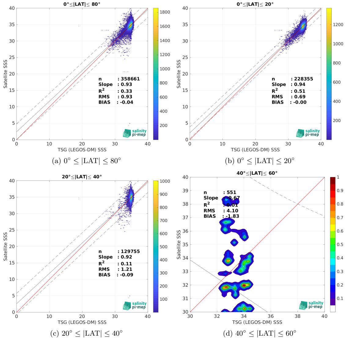
Figure 10: Contour maps of the concentration of SMOS SSS L2Q v331 - With FLAG (CMEMS-CATDS-CPDC) SSS (y-axis) versus TSG (LEGOS-DM) SSS (x-axis) at match-up pairs for different latitude bands. For each plot, the red line shows x=y . The black thin and dashed lines indicate a linear fit through the data cloud and the \pm 95\% confidence levels, respectively. The number match-up pairs n , the slope and R^2 coefficient of the linear fit, the root mean square (RMS) and the mean bias between satellite and in situ data are indicated for each latitude band in each plots.
