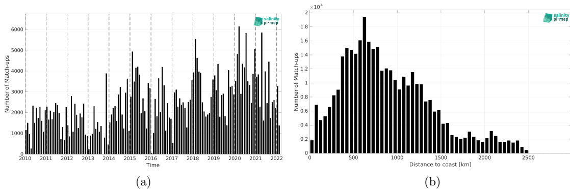
Figure 2: Number of match-ups between TSG (LEGOS-DM) and SMOS SSS L2Q v331 - With FLAG (CMEMS-CATDS-CPDC) SSS as a function of time (a) and as function of the distance to coast (b) over the North Pacific Ocean Pi-MEP region and for the full satellite product period.
