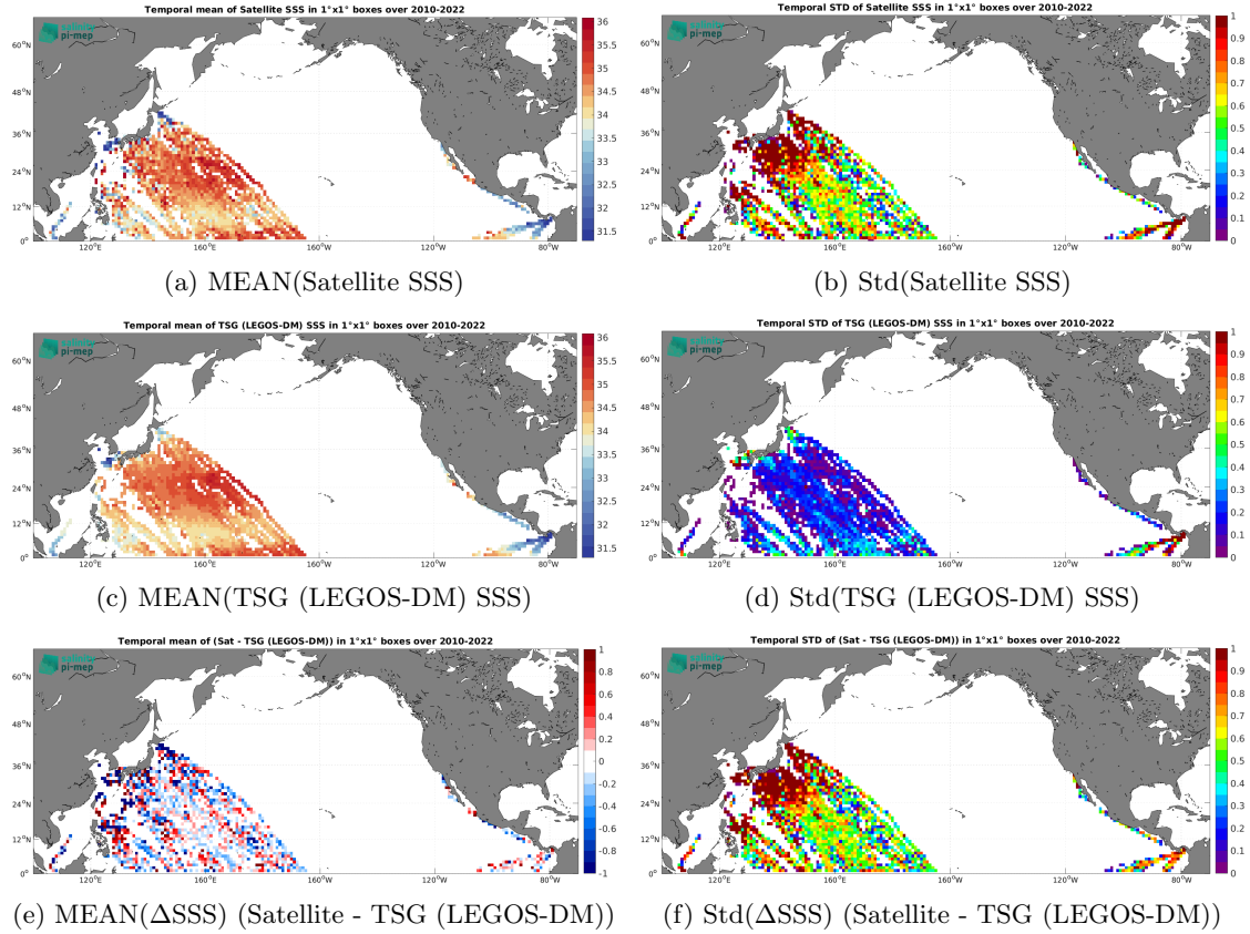
Figure 7: Temporal mean (left) and Std (right) of SSS from SMOS SSS L2Q v331 - With FLAG (CMEMS-CATDS-CPDC) (top), TSG (LEGOS-DM) (middle), and of \Delta\text{SSS} (Satellite - TSG (LEGOS-DM)). Only match-up pairs are used to generate these maps.
