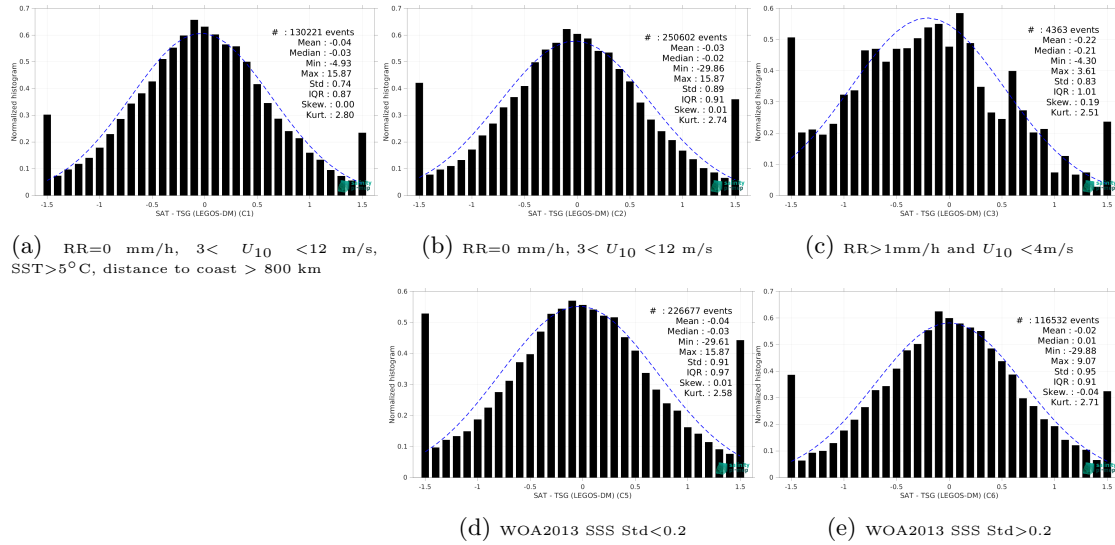
Figure 15: Normalized histogram of \Delta SSS (SMOS SSS L2Q v331 - With FLAG (CMEMS-CATDS-CPDC) - TSG (LEGOS-DM)) for 5 different subdatasets corresponding to: RR=0 mm/h, 3 < U_{10} < 12 m/s, SST>5°C, distance to coast > 800 km (a), RR=0 mm/h, 3 < U_{10} < 12 m/s (b), RR>1mm/h and U_{10} < 4 m/s (c), WOA2013 SSS Std<0.2 (d), WOA2013 SSS Std>0.2 (e).
