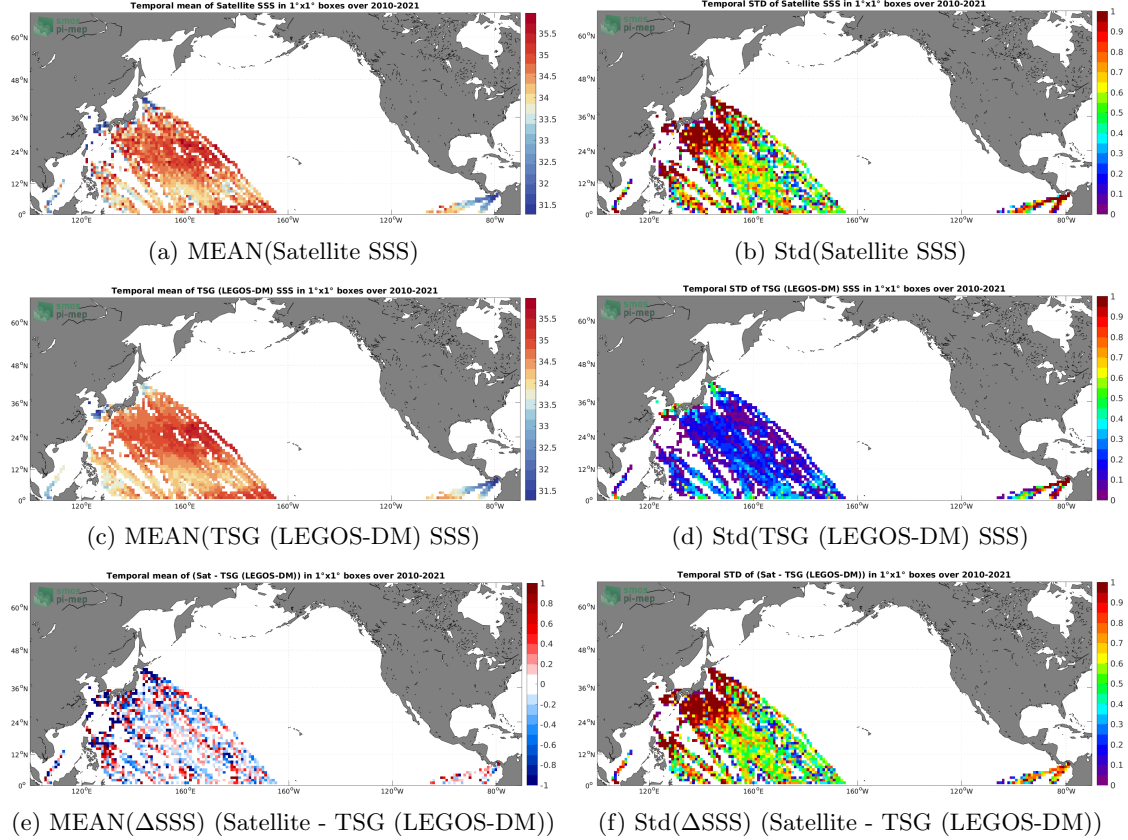
Figure 6: Temporal mean (left) and Std (right) of SSS from SMOS SSS L2Q v331 - With FLAG (CMEMS-CATDS-CPDC) (top), TSG (LEGOS-DM) (middle), and of \Delta\text{SSS} (Satellite - TSG (LEGOS-DM)). Only match-up pairs are used to generate these maps.
