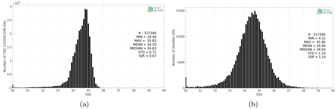
Figure 2: Histograms of SSS from TSG (LEGOS-DM) (a) and SMOS SSS L2Q v331 - With FLAG (CMEMS-CATDS-CPDC) (b) considering all match-up pairs per bins of 0.1 over the North Pacific Ocean Pi-MEP region and for the full satellite product period.
