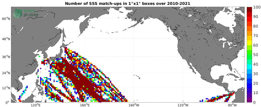
Figure 4: Number of SSS match-ups between TSG (LEGOS-DM) SSS and the SMOS SSS L2Q v331 - With FLAG (CMEMS-CATDS-CPDC) SSS product for the North Pacific Ocean Pi-MEP region over 1^\circ \times 1^\circ boxes and for the full satellite product period.
