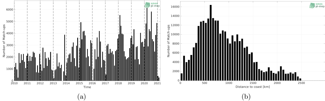
Figure 1: Number of match-ups between TSG (LEGOS-DM) and SMOS SSS L2Q v331 - With FLAG (CMEMS-CATDS-CPDC) SSS as a function of time (a) and as function of the distance to coast (b) over the North Pacific Ocean Pi-MEP region and for the full satellite product period.
