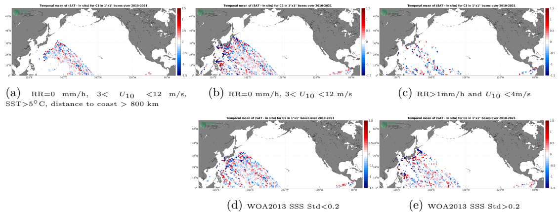
Figure 12: Temporal mean gridded over spatial boxes of size 1^\circ \times 1^\circ of \Delta SSS (SMOS SSS L2Q v331 - With FLAG (CMEMS-CATDS-CPDC) - TSG (LEGOS-DM)) for 5 different subdatasets corresponding to:RR=0 mm/h, 3 < U_{10} < 12 m/s, SST >5^\circ C, distance to coast > 800 km (a), RR=0 mm/h, 3 < U_{10} < 12 m/s (b), RR >1 mm/h and U_{10} < 4 m/s (c), WOA2013 SSS Std <0.2 (d), WOA2013 SSS Std >0.2 (e).
