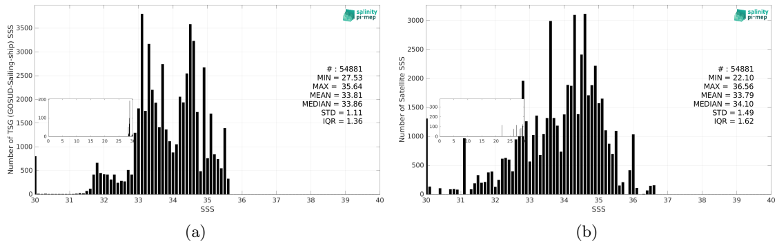
Figure 3: Histograms of SSS from TSG (GOSUD-Sailing-ship) (a) and SMOS SSS L2Q v331 - With FLAG (CMEMS-CATDS-CPDC) (b) considering all match-up pairs per bins of 0.1 over the North Pacific Ocean Pi-MEP region and for the full satellite product period.
