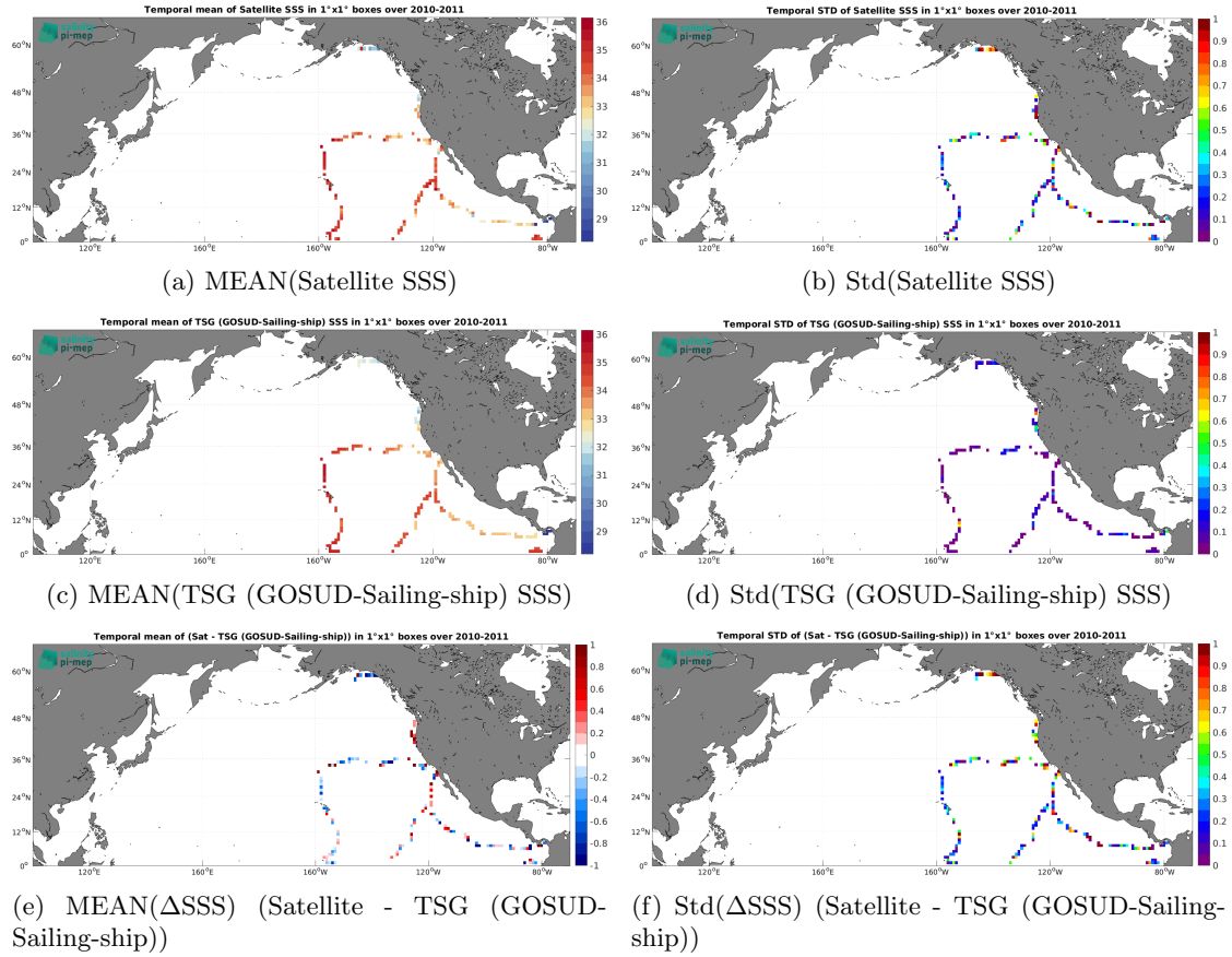
Figure 7: Temporal mean (left) and Std (right) of SSS from SMOS SSS L2Q v331 - With FLAG (CMEMS-CATDS-CPDC) (top), TSG (GOSUD-Sailing-ship) (middle), and of \Delta SSS (Satellite - TSG (GOSUD-Sailing-ship)). Only match-up pairs are used to generate these maps.
