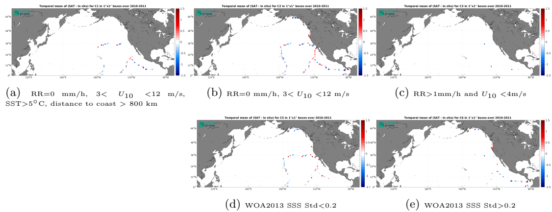
Figure 14: Temporal mean gridded over spatial boxes of size 1^\circ \times 1^\circ of \Delta SSS (SMOS SSS L2Q v331 - With FLAG (CMEMS-CATDS-CPDC) - TSG (GOSUD-Sailing-ship)) for 5 different subdatasets corresponding to:RR=0 mm/h, 3 < U_{10} < 12 m/s, SST >5^\circ\text{C} , distance to coast > 800 km (a), RR=0 mm/h, 3 < U_{10} < 12 m/s (b), RR >1 mm/h and U_{10} < 4 m/s (c), WOA2013 SSS Std <0.2 (d), WOA2013 SSS Std >0.2 (e).
