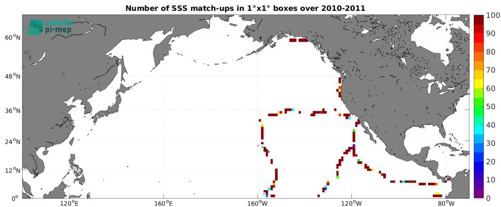
Figure 5: Number of SSS match-ups between TSG (GOSUD-Sailing-ship) SSS and the SMOS SSS L2Q v331 - With FLAG (CMEMS-CATDS-CPDC) SSS product for the North Pacific Ocean Pi-MEP region over 1^\circ \times 1^\circ boxes and for the full satellite product period.
