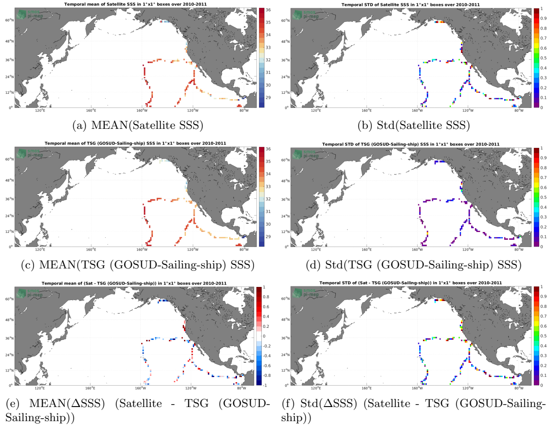
Figure 6: Temporal mean (left) and Std (right) of SSS from SMOS SSS L2Q v331 - With FLAG (CMEMS-CATDS-CPDC) (top), TSG (GOSUD-Sailing-ship) (middle), and of \Delta SSS (Satellite - TSG (GOSUD-Sailing-ship)). Only match-up pairs are used to generate these maps.
