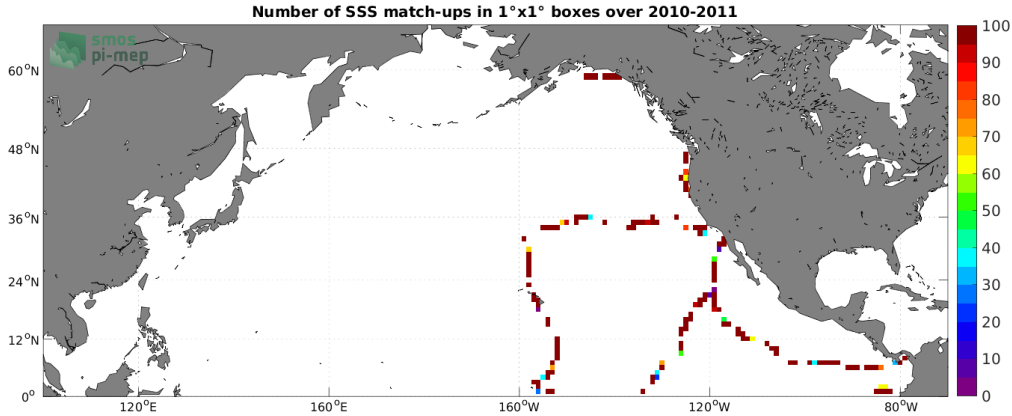
Figure 4: Number of SSS match-ups between TSG (GOSUD-Sailing-ship) SSS and the SMOS SSS L2Q v331 - With FLAG (CMEMS-CATDS-CPDC) SSS product for the North Pacific Ocean Pi-MEP region over 1^\circ \times 1^\circ boxes and for the full satellite product period.
