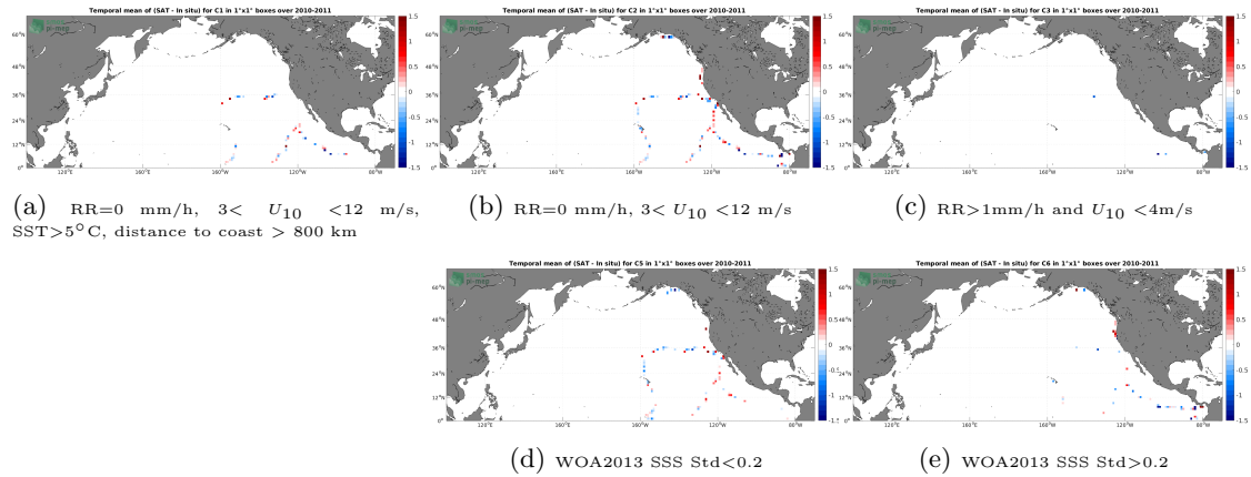
Figure 12: Temporal mean gridded over spatial boxes of size 1^\circ \times 1^\circ of \Delta\text{SSS} (SMOS SSS L2Q v331 - With FLAG (CMEMS-CATDS-CPDC) - TSG (GOSUD-Sailing-ship)) for 5 different subdatasets corresponding to:RR=0 mm/h, 3 < U_{10} < 12 m/s, SST >5^\circ\text{C} , distance to coast > 800 km (a), RR=0 mm/h, 3 < U_{10} < 12 m/s (b), RR >1 mm/h and U_{10} < 4 m/s (c), WOA2013 SSS Std <0.2 (d), WOA2013 SSS Std >0.2 (e).
