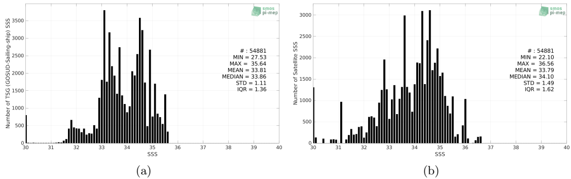
Figure 2: Histograms of SSS from TSG (GOSUD-Sailing-ship) (a) and SMOS SSS L2Q v331 - With FLAG (CMEMS-CATDS-CPDC) (b) considering all match-up pairs per bins of 0.1 over the North Pacific Ocean Pi-MEP region and for the full satellite product period.
