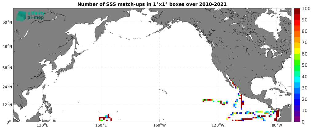
Figure 5: Number of SSS match-ups between TSG (GOSUD-Research-vessel) SSS and the SMOS SSS L2Q v331 - With FLAG (CMEMS-CATDS-CPDC) SSS product for the North Pacific Ocean Pi-MEP region over 1^\circ \times 1^\circ boxes and for the full satellite product period.
