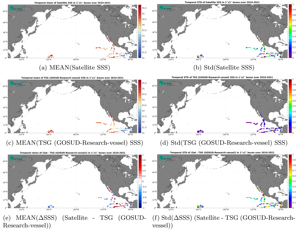
Figure 7: Temporal mean (left) and Std (right) of SSS from SMOS SSS L2Q v331 - With FLAG (CMEMS-CATDS-CPDC) (top), TSG (GOSUD-Research-vessel) (middle), and of \Delta SSS (Satellite - TSG (GOSUD-Research-vessel)). Only match-up pairs are used to generate these maps.
