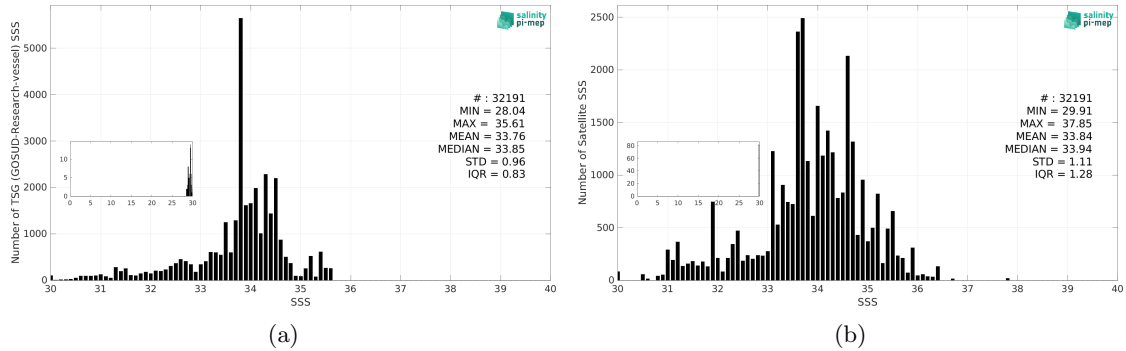
Figure 3: Histograms of SSS from TSG (GOSUD-Research-vessel) (a) and SMOS SSS L2Q v331 - With FLAG (CMEMS-CATDS-CPDC) (b) considering all match-up pairs per bins of 0.1 over the North Pacific Ocean Pi-MEP region and for the full satellite product period.
