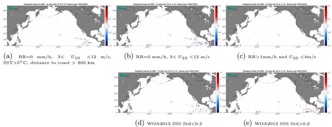
Figure 14: Temporal mean gridded over spatial boxes of size 1^\circ \times 1^\circ of \Delta SSS (SMOS SSS L2Q v331 - With FLAG (CMEMS-CATDS-CPDC) - TSG (GOSUD-Research-vessel)) for 5 different subdatasets corresponding to: RR=0 mm/h, 3 < U_{10} < 12 m/s, SST > 5°C, distance to coast > 800 km (a), RR=0 mm/h, 3 < U_{10} < 12 m/s (b), RR > 1mm/h and U_{10} < 4 m/s (c), WOA2013 SSS Std < 0.2 (d), WOA2013 SSS Std > 0.2 (e).
