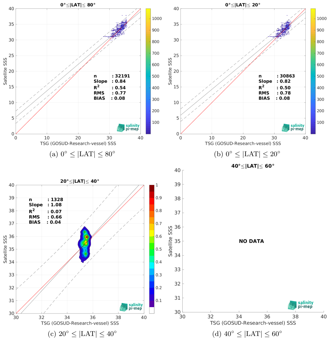
Figure 10: Contour maps of the concentration of SMOS SSS L2Q v331 - With FLAG (CMEMS-CATDS-CPDC) SSS (y-axis) versus TSG (GOSUD-Research-vessel) SSS (x-axis) at match-up pairs for different latitude bands. For each plot, the red line shows x=y . The black thin and dashed lines indicate a linear fit through the data cloud and the \pm 95\% confidence levels, respectively. The number match-up pairs n , the slope and R^2 coefficient of the linear fit, the root mean square (RMS) and the mean bias between satellite and in situ data are indicated for each latitude band in each plots.
