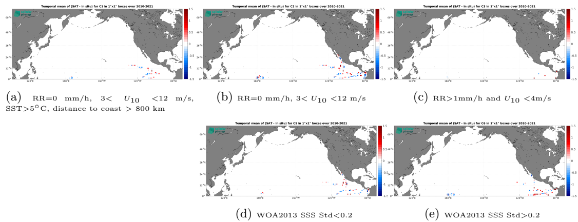
Figure 12: Temporal mean gridded over spatial boxes of size 1^\circ \times 1^\circ of \Delta SSS (SMOS SSS L2Q v331 - With FLAG (CMEMS-CATDS-CPDC) - TSG (GOSUD-Research-vessel)) for 5 different subdatasets corresponding to: RR=0 mm/h, 3 < U_{10} < 12 m/s, SST > 5°C, distance to coast > 800 km (a), RR=0 mm/h, 3 < U_{10} < 12 m/s (b), RR > 1 mm/h and U_{10} < 4 m/s (c), WOA2013 SSS Std < 0.2 (d), WOA2013 SSS Std > 0.2 (e).
