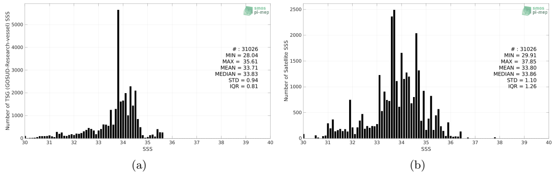
Figure 2: Histograms of SSS from TSG (GOSUD-Research-vessel) (a) and SMOS SSS L2Q v331 - With FLAG (CMEMS-CATDS-CPDC) (b) considering all match-up pairs per bins of 0.1 over the North Pacific Ocean Pi-MEP region and for the full satellite product period.
