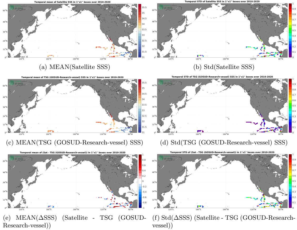
Figure 6: Temporal mean (left) and Std (right) of SSS from SMOS SSS L2Q v331 - With FLAG (CMEMS-CATDS-CPDC) (top), TSG (GOSUD-Research-vessel) (middle), and of \Delta SSS (Satellite - TSG (GOSUD-Research-vessel)). Only match-up pairs are used to generate these maps.
