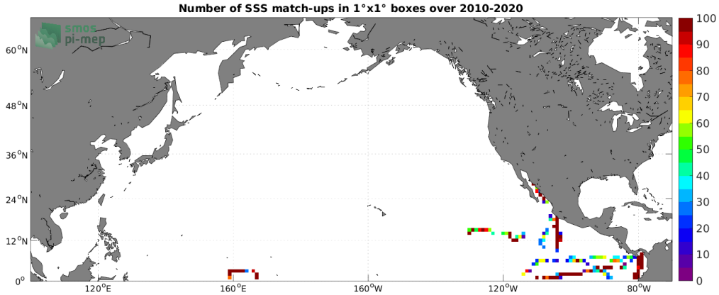
Figure 4: Number of SSS match-ups between TSG (GOSUD-Research-vessel) SSS and the SMOS SSS L2Q v331 - With FLAG (CMEMS-CATDS-CPDC) SSS product for the North Pacific Ocean Pi-MEP region over 1^\circ \times 1^\circ boxes and for the full satellite product period.
