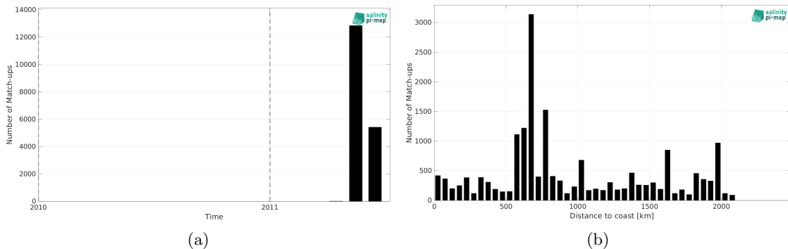
Figure 2: Number of match-ups between TSG (CSIC-UTM) and SMOS SSS L2Q v331 - With FLAG (CMEMS-CATDS-CPDC) SSS as a function of time (a) and as function of the distance to coast (b) over the North Pacific Ocean Pi-MEP region and for the full satellite product period.
