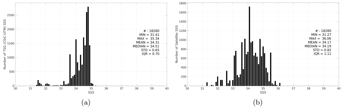
Figure 3: Histograms of SSS from TSG (CSIC-UTM) (a) and SMOS SSS L2Q v331 - With FLAG (CMEMS-CATDS-CPDC) (b) considering all match-up pairs per bins of 0.1 over the North Pacific Ocean Pi-MEP region and for the full satellite product period.
