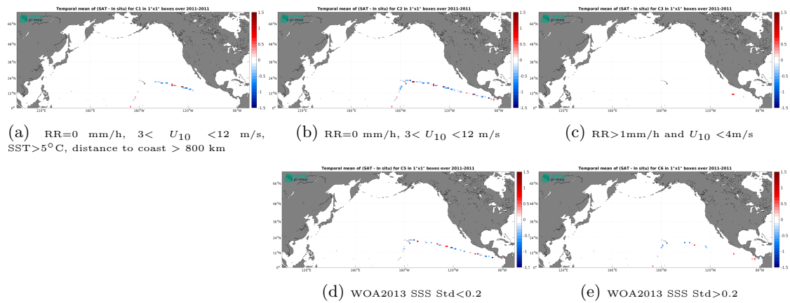
Figure 14: Temporal mean gridded over spatial boxes of size 1^\circ \times 1^\circ of \Delta SSS (SMOS SSS L2Q v331 - With FLAG (CMEMS-CATDS-CPDC) - TSG (CSIC-UTM)) for 5 different subdatasets corresponding to:RR=0 mm/h, 3 < U_{10} < 12 m/s, SST >5^\circ\text{C} , distance to coast > 800 km (a), RR=0 mm/h, 3 < U_{10} < 12 m/s (b), RR >1 mm/h and U_{10} < 4 m/s (c), WOA2013 SSS Std <0.2 (d), WOA2013 SSS Std >0.2 (e).
