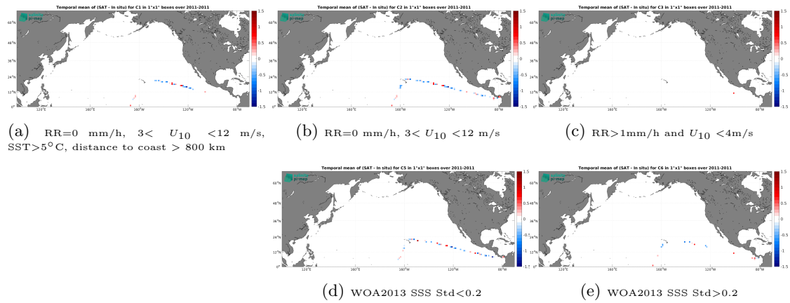
Figure 12: Temporal mean gridded over spatial boxes of size 1^{\circ}\times 1^{\circ} of \Delta\text{SSS} (SMOS SSS L2Q v331 - With FLAG (CMEMS-CATDS-CPDC) - TSG (CSIC-UTM)) for 5 different subdatasets corresponding to:RR=0 mm/h, 3 < U_{10} < 12 m/s, SST >5^{\circ}\text{C} , distance to coast > 800 km (a), RR=0 mm/h, 3 < U_{10} < 12 m/s (b), RR >1 mm/h and U_{10} < 4 m/s (c), WOA2013 SSS Std <0.2 (d), WOA2013 SSS Std >0.2 (e).
