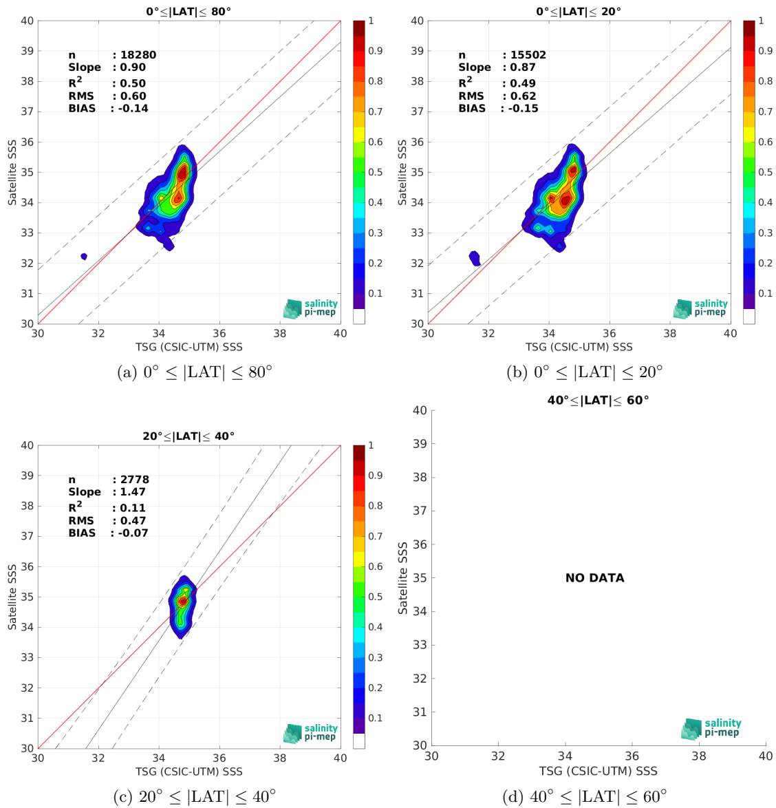
Figure 9: Contour maps of the concentration of SMOS SSS L2Q v331 - With FLAG (CMEMS-CATDS-CPDC) SSS (y-axis) versus TSG (CSIC-UTM) SSS (x-axis) at match-up pairs for different latitude bands. For each plot, the red line shows x=y . The black thin and dashed lines indicate a linear fit through the data cloud and the \pm 95\% confidence levels, respectively. The number match-up pairs n , the slope and R^2 coefficient of the linear fit, the root mean square (RMS) and the mean bias between satellite and in situ data are indicated for each latitude band in each plots.
