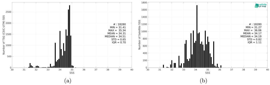
Figure 2: Histograms of SSS from TSG (CSIC-UTM) (a) and SMOS SSS L2Q v331 - With FLAG (CMEMS-CATDS-CPDC) (b) considering all match-up pairs per bins of 0.1 over the North Pacific Ocean Pi-MEP region and for the full satellite product period.
