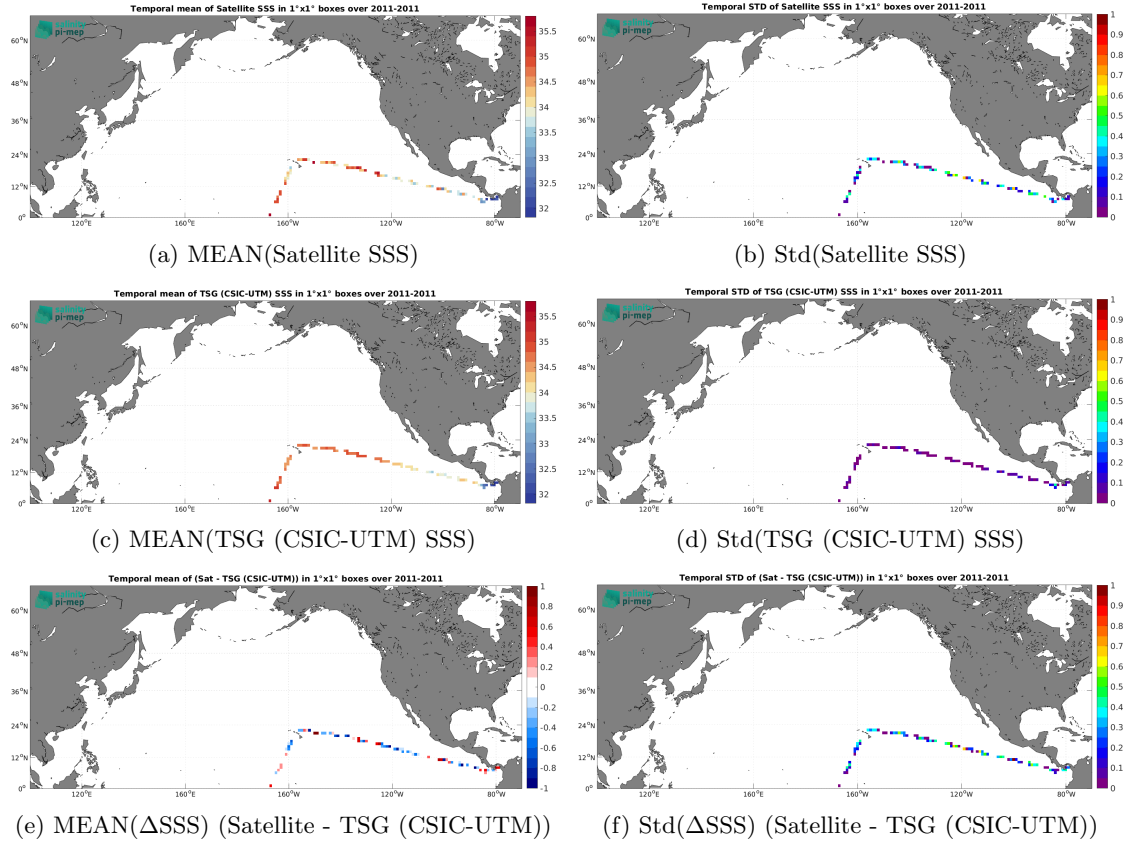
Figure 6: Temporal mean (left) and Std (right) of SSS from SMOS SSS L2Q v331 - With FLAG (CMEMS-CATDS-CPDC) (top), TSG (CSIC-UTM) (middle), and of \Delta\text{SSS} (Satellite - TSG (CSIC-UTM)). Only match-up pairs are used to generate these maps.
