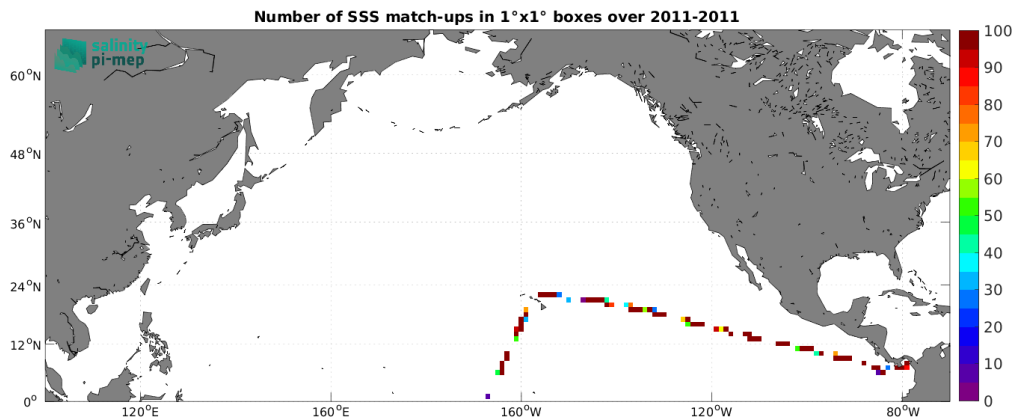
Figure 4: Number of SSS match-ups between TSG (CSIC-UTM) SSS and the SMOS SSS L2Q v331 - With FLAG (CMEMS-CATDS-CPDC) SSS product for the North Pacific Ocean Pi-MEP region over 1^\circ \times 1^\circ boxes and for the full satellite product period.
