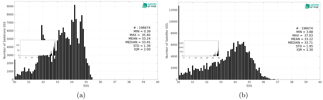
Figure 3: Histograms of SSS from Saildrone (a) and SMOS SSS L2Q v331 - With FLAG (CMEMS-CATDS-CPDC) (b) considering all match-up pairs per bins of 0.1 over the North Pacific Ocean Pi-MEP region and for the full satellite product period.
