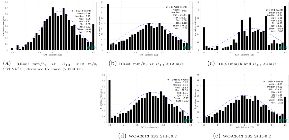
Figure 15: Normalized histogram of \Delta SSS (SMOS SSS L2Q v331 - With FLAG (CMEMS-CATDS-CPDC) - Sairdrone) for 5 different subdatasets corresponding to: RR=0 mm/h, 3 < U_{10} < 12 m/s, SST > 5°C, distance to coast > 800 km (a), RR=0 mm/h, 3 < U_{10} < 12 m/s (b), RR > 1mm/h and U_{10} < 4 m/s (c), WOA2013 SSS Std < 0.2 (d), WOA2013 SSS Std > 0.2 (e).
