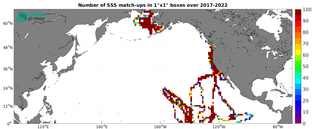
Figure 5: Number of SSS match-ups between Saildrone SSS and the SMOS SSS L2Q v331 - With FLAG (CMEMS-CATDS-CPDC) SSS product for the North Pacific Ocean Pi-MEP region over 1^\circ \times 1^\circ boxes and for the full satellite product period.
