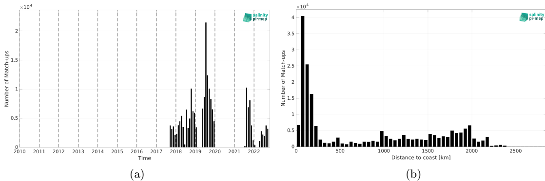
Figure 2: Number of match-ups between Saildrone and SMOS SSS L2Q v331 - With FLAG (CMEMS-CATDS-CPDC) SSS as a function of time (a) and as function of the distance to coast (b) over the North Pacific Ocean Pi-MEP region and for the full satellite product period.
