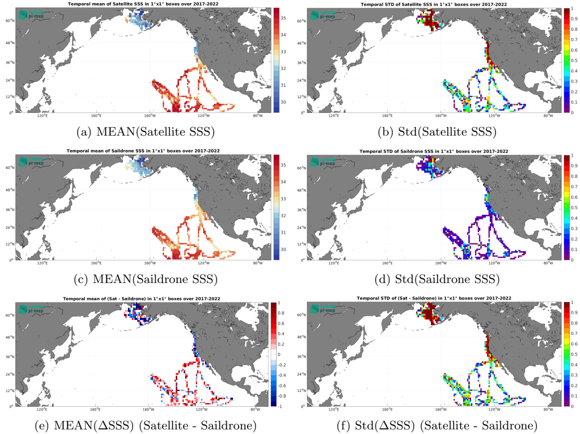
Figure 7: Temporal mean (left) and Std (right) of SSS from SMOS SSS L2Q v331 - With FLAG (CMEMS-CATDS-CPDC) (top), Saildrone (middle), and of \Delta SSS (Satellite - Saildrone). Only match-up pairs are used to generate these maps.
