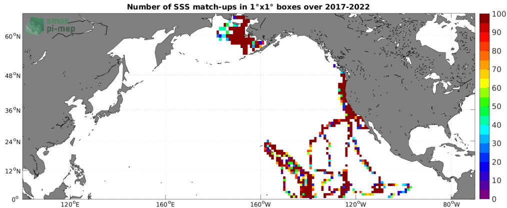
Figure 4: Number of SSS match-ups between Saildrone SSS and the SMOS SSS L2Q v331 - With FLAG (CMEMS-CATDS-CPDC) SSS product for the North Pacific Ocean Pi-MEP region over 1^\circ \times 1^\circ boxes and for the full satellite product period.
