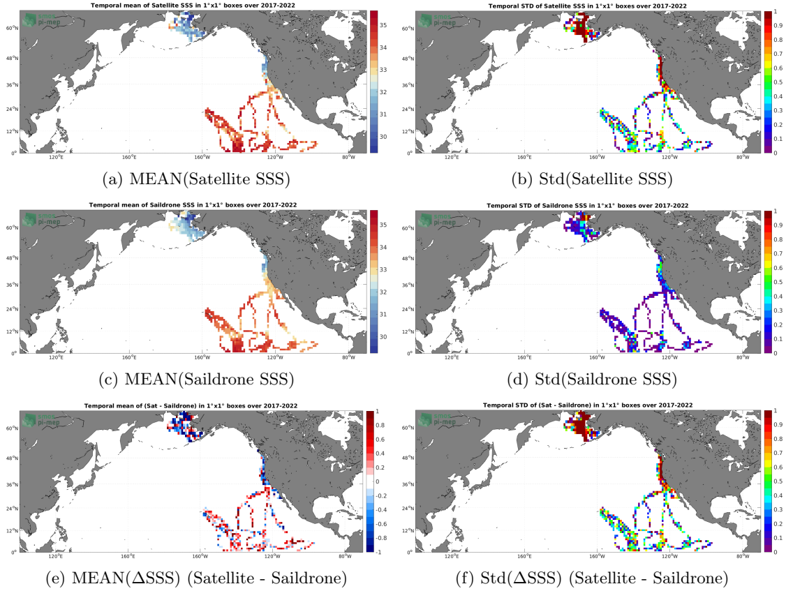
Figure 6: Temporal mean (left) and Std (right) of SSS from SMOS SSS L2Q v331 - With FLAG (CMEMS-CATDS-CPDC) (top), Saildrone (middle), and of \Delta SSS (Satellite - Saildrone). Only match-up pairs are used to generate these maps.
