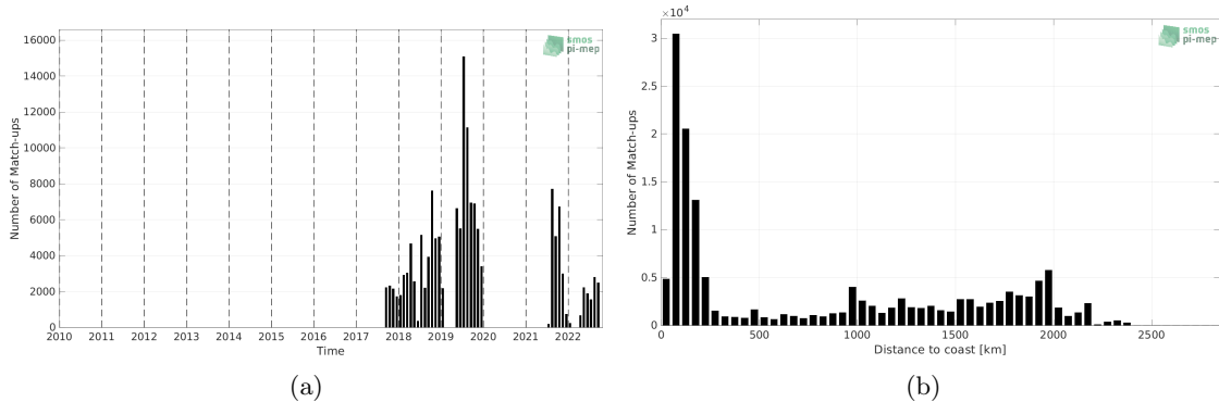
Figure 1: Number of match-ups between Saildrone and SMOS SSS L2Q v331 - With FLAG (CMEMS-CATDS-CPDC) SSS as a function of time (a) and as function of the distance to coast (b) over the North Pacific Ocean Pi-MEP region and for the full satellite product period.
