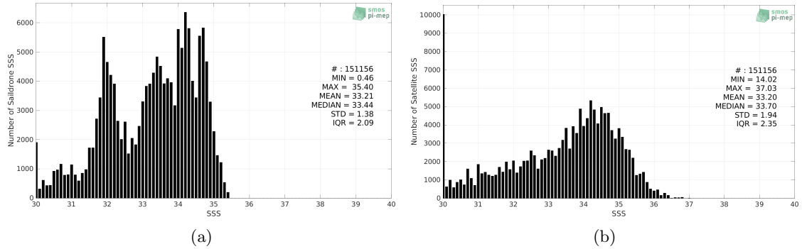
Figure 2: Histograms of SSS from Saildrone (a) and SMOS SSS L2Q v331 - With FLAG (CMEMS-CATDS-CPDC) (b) considering all match-up pairs per bins of 0.1 over the North Pacific Ocean Pi-MEP region and for the full satellite product period.
