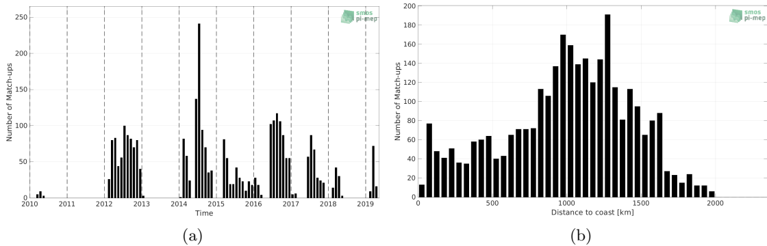
Figure 1: Number of match-ups between Marine mammals and SMOS SSS L2Q v331 - With FLAG (CMEMS-CATDS-CPDC) SSS as a function of time (a) and as function of the distance to coast (b) over the North Pacific Ocean Pi-MEP region and for the full satellite product period.
