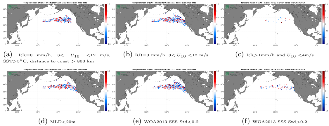
Figure 12: Temporal mean gridded over spatial boxes of size 1^{\circ}\times 1^{\circ} of \Delta\text{SSS} (SMOS SSS L2Q v331 - With FLAG (CMEMS-CATDS-CPDC) - Marine mammals) for 6 different subdatasets corresponding to:RR=0 mm/h, 3 < U_{10} < 12 m/s, SST >5^{\circ}\text{C} , distance to coast > 800 km (a), RR=0 mm/h, 3 < U_{10} < 12 m/s (b), RR >1 mm/h and U_{10} < 4 m/s (c),MLD <20 m (d),WOA2013 SSS Std <0.2 (e),WOA2013 SSS Std >0.2 (f).
