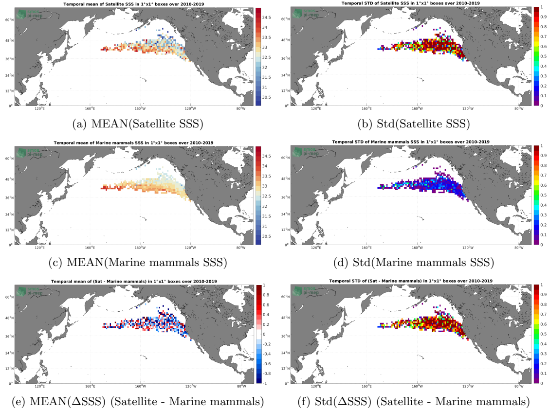
Figure 6: Temporal mean (left) and Std (right) of SSS from SMOS SSS L2Q v331 - With FLAG (CMEMS-CATDS-CPDC) (top), Marine mammals (middle), and of \Delta SSS (Satellite - Marine mammals). Only match-up pairs are used to generate these maps.
