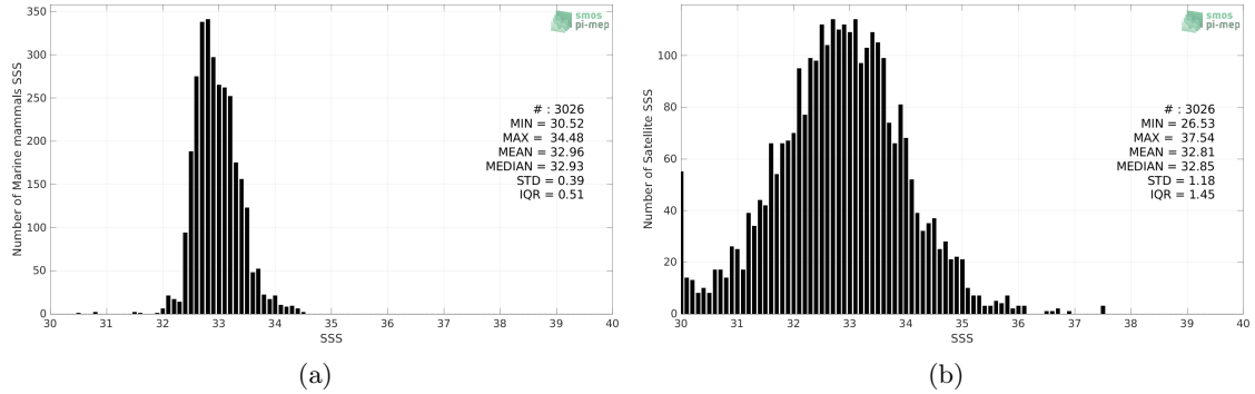
Figure 2: Histograms of SSS from Marine mammals (a) and SMOS SSS L2Q v331 - With FLAG (CMEMS-CATDS-CPDC) (b) considering all match-up pairs per bins of 0.1 over the North Pacific Ocean Pi-MEP region and for the full satellite product period.
