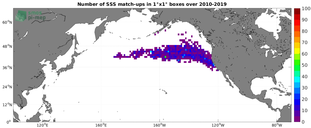
Figure 4: Number of SSS match-ups between Marine mammals SSS and the SMOS SSS L2Q v331 - With FLAG (CMEMS-CATDS-CPDC) SSS product for the North Pacific Ocean Pi-MEP region over 1^\circ \times 1^\circ boxes and for the full satellite product period.
