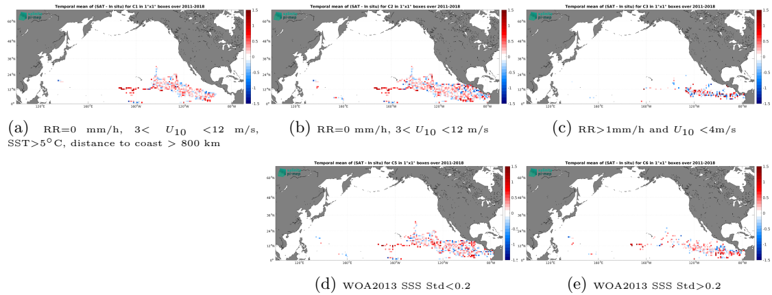
Figure 13: Temporal mean gridded over spatial boxes of size 1^\circ \times 1^\circ of \Delta\text{SSS} (SMOS SSS L2Q v331 - With FLAG (CMEMS-CATDS-CPDC) - Surface drifters) for 5 different subdatasets corresponding to:RR=0 mm/h, 3 < U_{10} < 12 m/s, SST >5^\circ\text{C} , distance to coast > 800 km (a), RR=0 mm/h, 3 < U_{10} < 12 m/s (b), RR >1 mm/h and U_{10} < 4 m/s (c), WOA2013 SSS Std <0.2 (d), WOA2013 SSS Std >0.2 (e).
