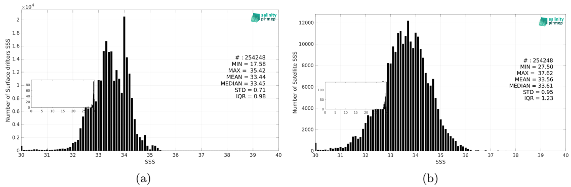
Figure 3: Histograms of SSS from Surface drifters (a) and SMOS SSS L2Q v331 - With FLAG (CMEMS-CATDS-CPDC) (b) considering all match-up pairs per bins of 0.1 over the North Pacific Ocean Pi-MEP region and for the full satellite product period.
