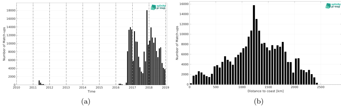
Figure 2: Number of match-ups between Surface drifters and SMOS SSS L2Q v331 - With FLAG (CMEMS-CATDS-CPDC) SSS as a function of time (a) and as function of the distance to coast (b) over the North Pacific Ocean Pi-MEP region and for the full satellite product period.
