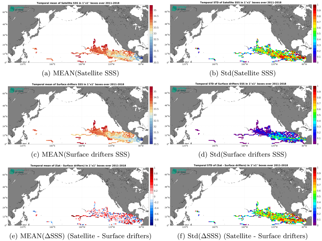
Figure 6: Temporal mean (left) and Std (right) of SSS from SMOS SSS L2Q v331 - With FLAG (CMEMS-CATDS-CPDC) (top), Surface drifters (middle), and of \Delta SSS (Satellite - Surface drifters). Only match-up pairs are used to generate these maps.
