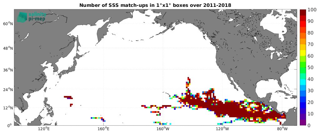
Figure 4: Number of SSS match-ups between Surface drifters SSS and the SMOS SSS L2Q v331 - With FLAG (CMEMS-CATDS-CPDC) SSS product for the North Pacific Ocean Pi-MEP region over 1^\circ \times 1^\circ boxes and for the full satellite product period.
