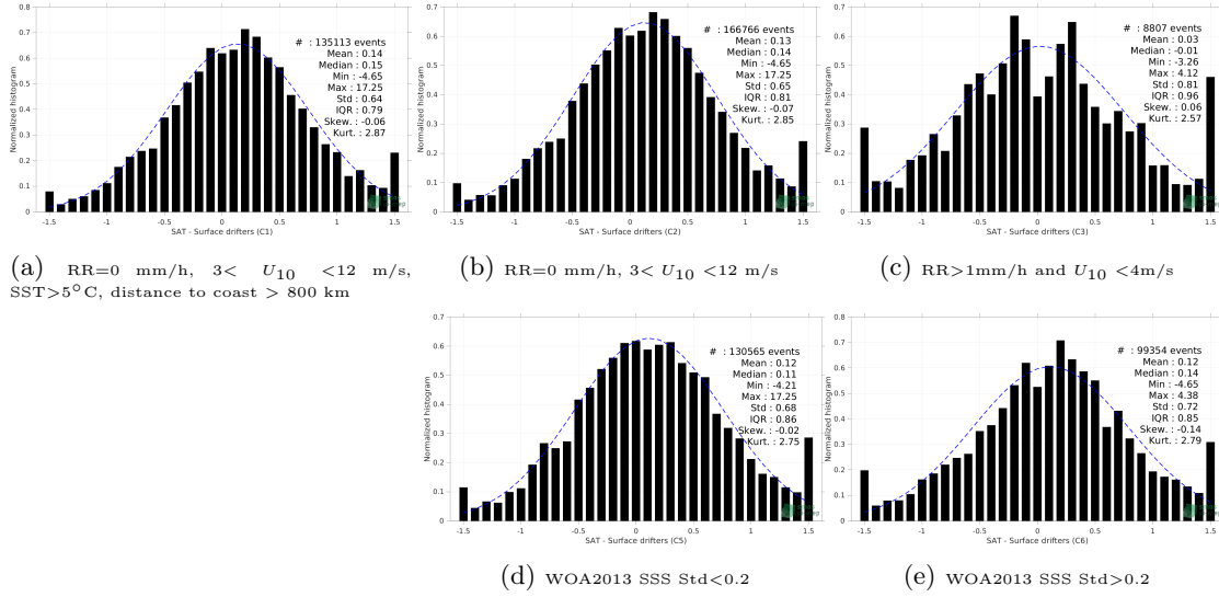
Figure 12: Normalized histogram of \Delta SSS (SMOS SSS L2Q v331 - With FLAG (CMEMS-CATDS-CPDC) - Surface drifters) for 5 different subdatasets corresponding to: RR=0 mm/h, 3 < U_{10} < 12 m/s, SST > 5°C, distance to coast > 800 km (a), RR=0 mm/h, 3 < U_{10} < 12 m/s (b), RR > 1mm/h and U_{10} < 4 m/s (c), WOA2013 SSS Std < 0.2 (d), WOA2013 SSS Std > 0.2 (e).
