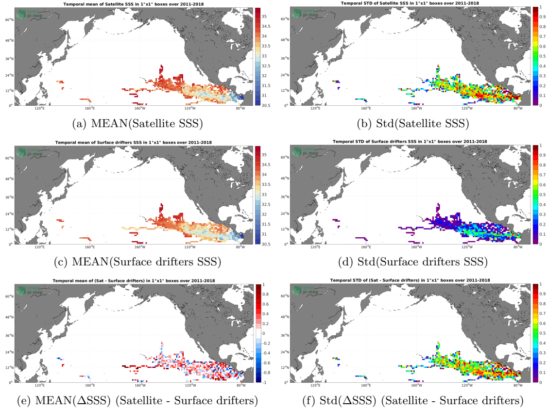
Figure 5: Temporal mean (left) and Std (right) of SSS from SMOS SSS L2Q v331 - With FLAG (CMEMS-CATDS-CPDC) (top), Surface drifters (middle), and of \Delta SSS (Satellite - Surface drifters). Only match-up pairs are used to generate these maps.
