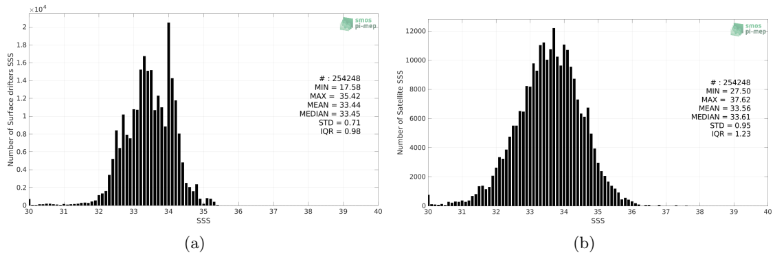
Figure 2: Histograms of SSS from Surface drifters (a) and SMOS SSS L2Q v331 - With FLAG (CMEMS-CATDS-CPDC) (b) considering all match-up pairs per bins of 0.1 over the North Pacific Ocean Pi-MEP region and for the full satellite product period.
