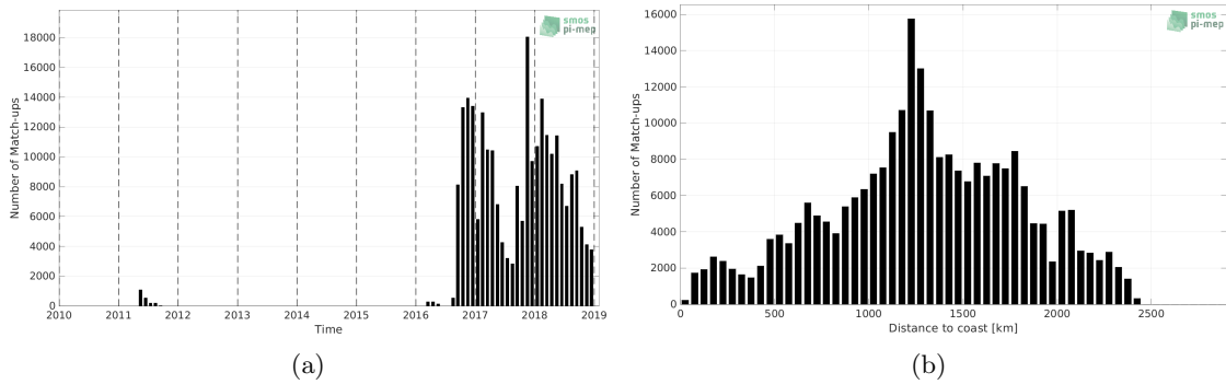
Figure 1: Number of match-ups between Surface drifters and SMOS SSS L2Q v331 - With FLAG (CMEMS-CATDS-CPDC) SSS as a function of time (a) and as function of the distance to coast (b) over the North Pacific Ocean Pi-MEP region and for the full satellite product period.
