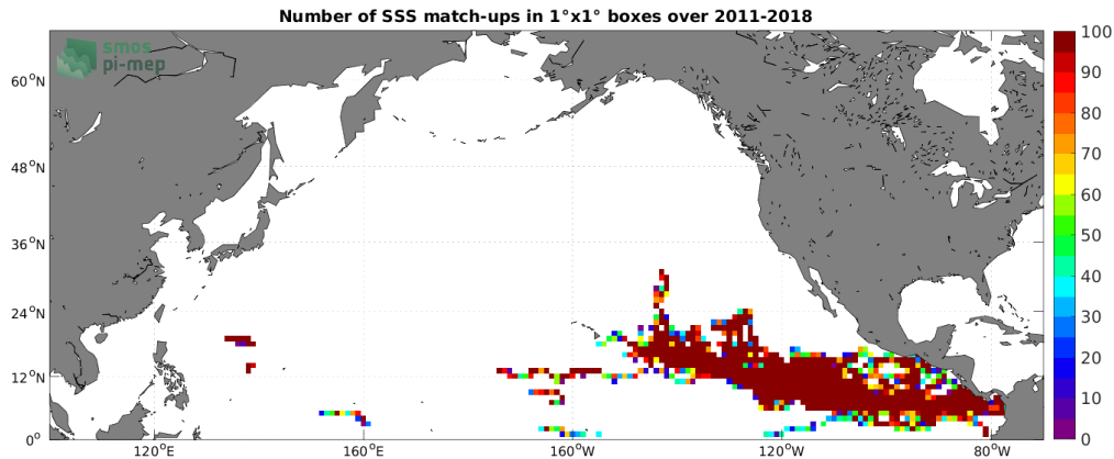
Figure 3: Number of SSS match-ups between Surface drifters SSS and the SMOS SSS L2Q v331 - With FLAG (CMEMS-CATDS-CPDC) SSS product for the North Pacific Ocean Pi-MEP region over 1^\circ \times 1^\circ boxes and for the full satellite product period.
