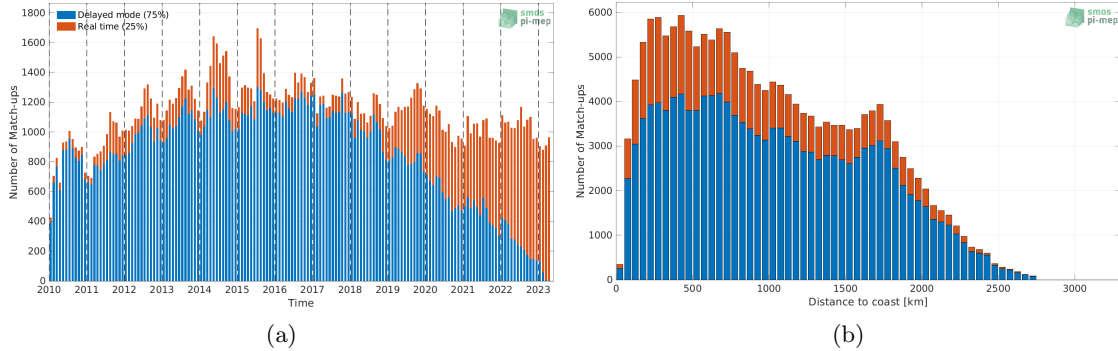
Figure 1: Number of match-ups between Argo and SMOS SSS L2Q v331 - With FLAG (CMEMS-CATDS-CPDC) SSS as a function of time (a) and as function of the distance to coast (b) over the North Pacific Ocean Pi-MEP region and for the full satellite product period.
