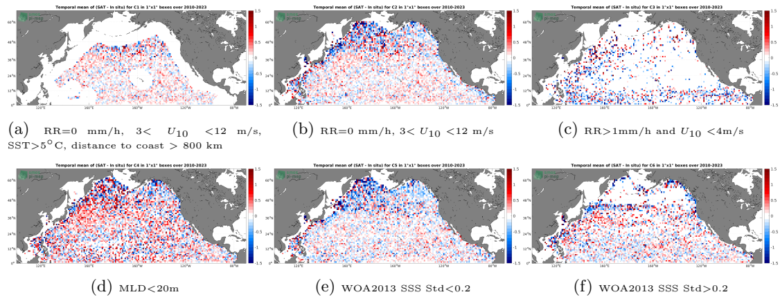
Figure 12: Temporal mean gridded over spatial boxes of size 1^\circ \times 1^\circ of \Delta SSS (SMOS SSS L2Q v331 - With FLAG (CMEMS-CATDS-CPDC) - Argo) for 6 different subdatasets corresponding to:RR=0 mm/h, 3 < U_{10} < 12 m/s, SST >5^\circ C, distance to coast > 800 km (a), RR=0 mm/h, 3 < U_{10} < 12 m/s (b), RR >1 mm/h and U_{10} < 4 m/s (c),MLD <20 m (d),WOA2013 SSS Std <0.2 (e),WOA2013 SSS Std >0.2 (f).
