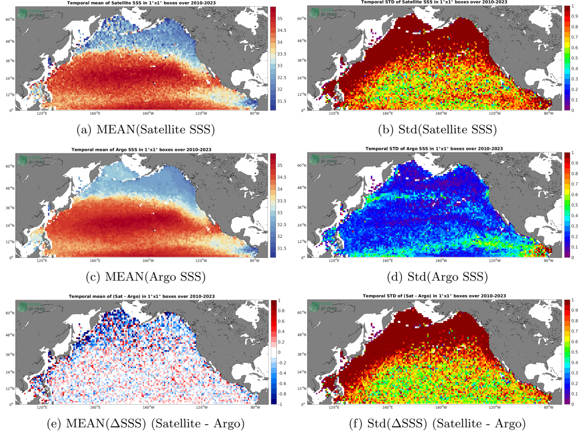
Figure 6: Temporal mean (left) and Std (right) of SSS from SMOS SSS L2Q v331 - With FLAG (CMEMS-CATDS-CPDC) (top), Argo (middle), and of \Delta\text{SSS} (Satellite - Argo). Only match-up pairs are used to generate these maps.
