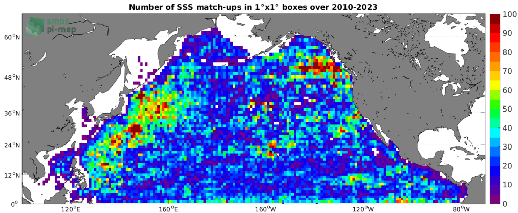
Figure 4: Number of SSS match-ups between Argo SSS and the SMOS SSS L2Q v331 - With FLAG (CMEMS-CATDS-CPDC) SSS product for the North Pacific Ocean Pi-MEP region over 1^\circ \times 1^\circ boxes and for the full satellite product period.
