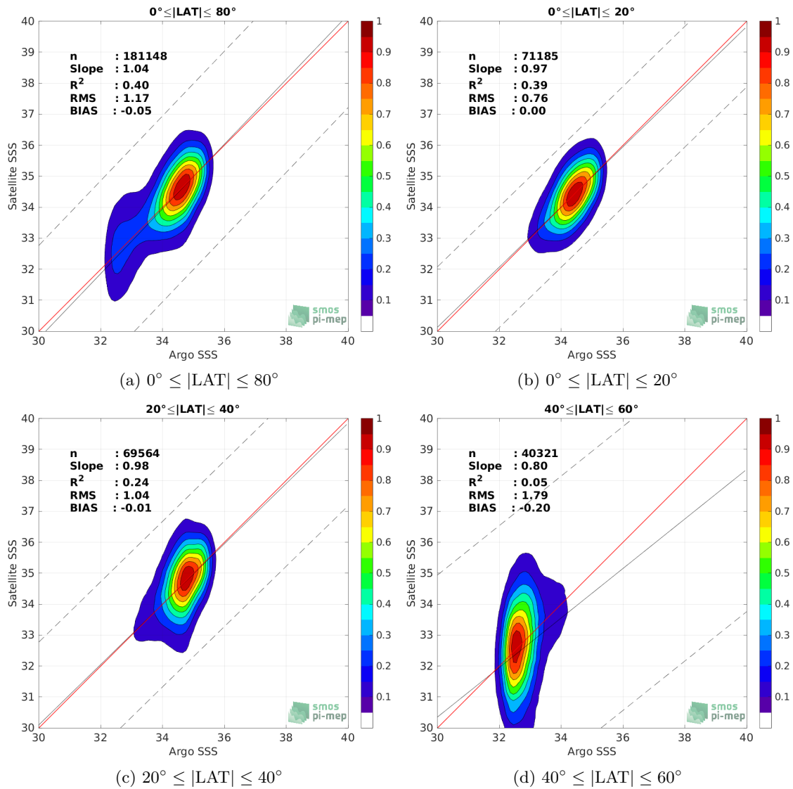
Figure 9: Contour maps of the concentration of SMOS SSS L2Q v331 - With FLAG (CMEMS-CATDS-CPDC) SSS (y-axis) versus Argo SSS (x-axis) at match-up pairs for different latitude bands. For each plot, the red line shows x=y . The black thin and dashed lines indicate a linear fit through the data cloud and the \pm 95\% confidence levels, respectively. The number match-up pairs n , the slope and R^2 coefficient of the linear fit, the root mean square (RMS) and the mean bias between satellite and in situ data are indicated for each latitude band in each plots.
