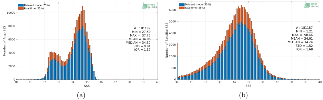
Figure 2: Histograms of SSS from Argo (a) and SMOS SSS L2Q v331 - With FLAG (CMEMS-CATDS-CPDC) (b) considering all match-up pairs per bins of 0.1 over the North Pacific Ocean Pi-MEP region and for the full satellite product period.
