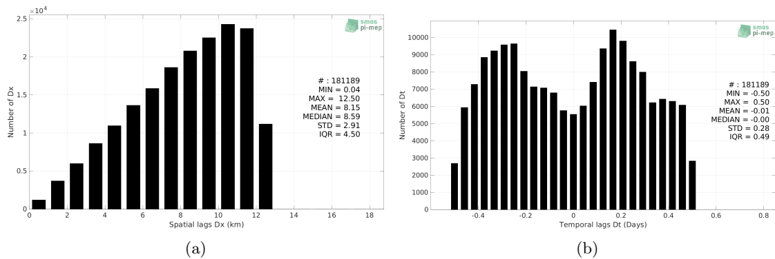
Figure 5: Histograms of the spatial (a) and temporal (b) lags between the location/time of the Argo measurement and the date of the corresponding SMOS SSS L2Q v331 - With FLAG (CMEMS-CATDS-CPDC) SSS pixel.
