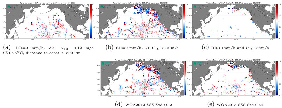
Figure 14: Temporal mean gridded over spatial boxes of size 1^\circ \times 1^\circ of \Delta SSS (SMOS SSS L2Q v331 - No FLAG (CMEMS-CATDS-CPDC) - TSG (SAMOS)) for 5 different subdatasets corresponding to: RR=0 mm/h, 3 < U_{10} < 12 m/s, SST > 5°C, distance to coast > 800 km (a), RR=0 mm/h, 3 < U_{10} < 12 m/s (b), RR > 1mm/h and U_{10} < 4 m/s (c), WOA2013 SSS Std < 0.2 (d), WOA2013 SSS Std > 0.2 (e).
