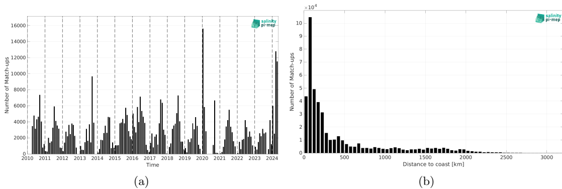
Figure 2: Number of match-ups between TSG (SAMOS) and SMOS SSS L2Q v331 - No FLAG (CMEMS-CATDS-CPDC) SSS as a function of time (a) and as function of the distance to coast (b) over the North Pacific Ocean Pi-MEP region and for the full satellite product period.
