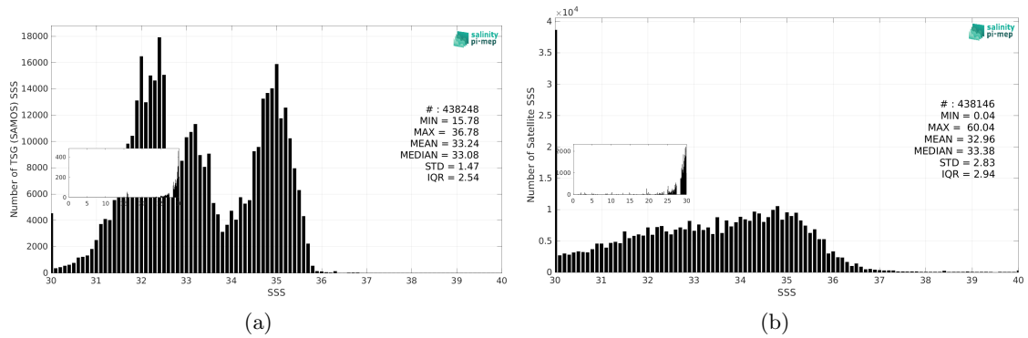
Figure 3: Histograms of SSS from TSG (SAMOS) (a) and SMOS SSS L2Q v331 - No FLAG (CMEMS-CATDS-CPDC) (b) considering all match-up pairs per bins of 0.1 over the North Pacific Ocean Pi-MEP region and for the full satellite product period.
