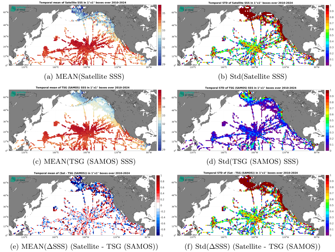
Figure 7: Temporal mean (left) and Std (right) of SSS from SMOS SSS L2Q v331 - No FLAG (CMEMS-CATDS-CPDC) (top), TSG (SAMOS) (middle), and of \Delta SSS (Satellite - TSG (SAMOS)). Only match-up pairs are used to generate these maps.
