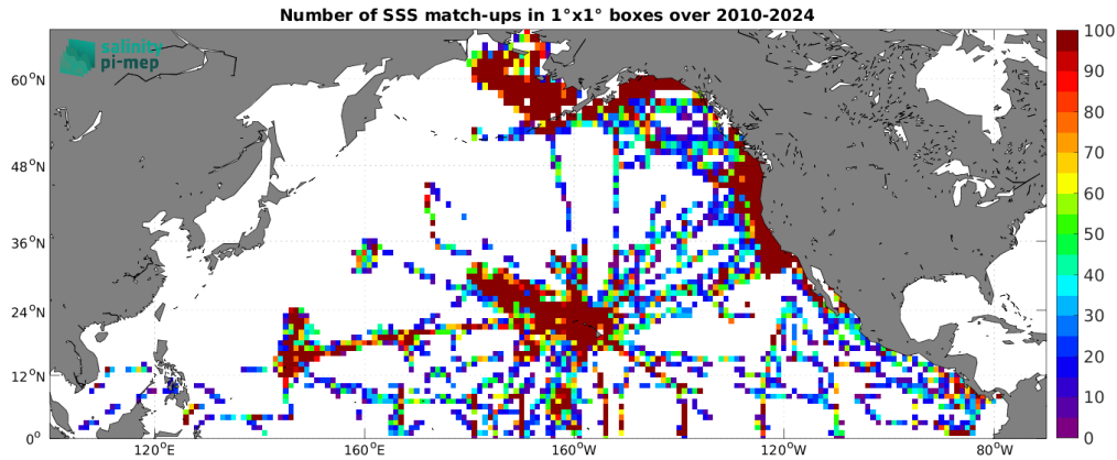
Figure 5: Number of SSS match-ups between TSG (SAMOS) SSS and the SMOS SSS L2Q v331 - No FLAG (CMEMS-CATDS-CPDC) SSS product for the North Pacific Ocean Pi-MEP region over 1^\circ \times 1^\circ boxes and for the full satellite product period.
