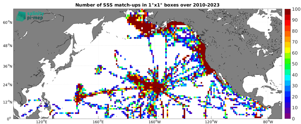
Figure 4: Number of SSS match-ups between TSG (SAMOS) SSS and the SMOS SSS L2Q v331 - No FLAG (CMEMS-CATDS-CPDC) SSS product for the North Pacific Ocean Pi-MEP region over 1^\circ \times 1^\circ boxes and for the full satellite product period.
