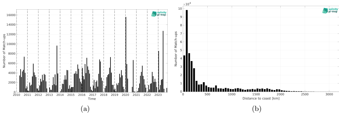
Figure 1: Number of match-ups between TSG (SAMOS) and SMOS SSS L2Q v331 - No FLAG (CMEMS-CATDS-CPDC) SSS as a function of time (a) and as function of the distance to coast (b) over the North Pacific Ocean Pi-MEP region and for the full satellite product period.
