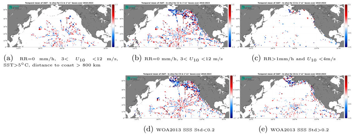
Figure 12: Temporal mean gridded over spatial boxes of size 1^\circ \times 1^\circ of \Delta SSS (SMOS SSS L2Q v331 - No FLAG (CMEMS-CATDS-CPDC) - TSG (SAMOS)) for 5 different subdatasets corresponding to:RR=0 mm/h, 3 < U_{10} < 12 m/s, SST >5^\circ C, distance to coast > 800 km (a), RR=0 mm/h, 3 < U_{10} < 12 m/s (b), RR >1 mm/h and U_{10} < 4 m/s (c), WOA2013 SSS Std <0.2 (d), WOA2013 SSS Std >0.2 (e).
