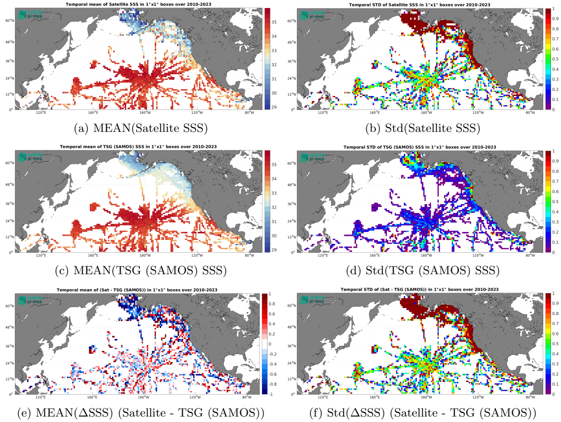
Figure 6: Temporal mean (left) and Std (right) of SSS from SMOS SSS L2Q v331 - No FLAG (CMEMS-CATDS-CPDC) (top), TSG (SAMOS) (middle), and of \Delta SSS (Satellite - TSG (SAMOS)). Only match-up pairs are used to generate these maps.
