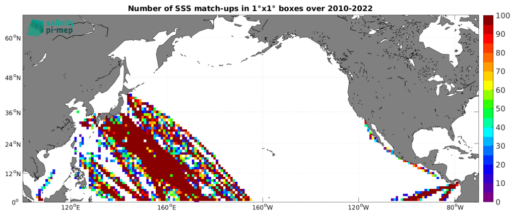
Figure 5: Number of SSS match-ups between TSG (LEGOS-DM) SSS and the SMOS SSS L2Q v331 - No FLAG (CMEMS-CATDS-CPDC) SSS product for the North Pacific Ocean Pi-MEP region over 1^\circ \times 1^\circ boxes and for the full satellite product period.
