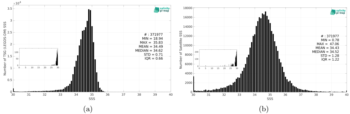
Figure 3: Histograms of SSS from TSG (LEGOS-DM) (a) and SMOS SSS L2Q v331 - No FLAG (CMEMS-CATDS-CPDC) (b) considering all match-up pairs per bins of 0.1 over the North Pacific Ocean Pi-MEP region and for the full satellite product period.
