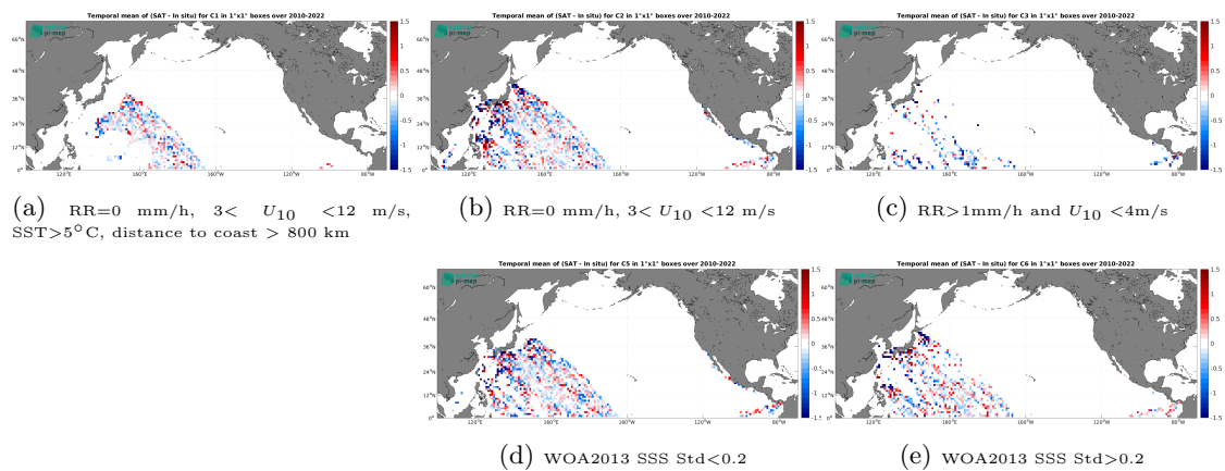
Figure 14: Temporal mean gridded over spatial boxes of size 1^\circ \times 1^\circ of \Delta\text{SSS} (SMOS SSS L2Q v331 - No FLAG (CMEMS-CATDS-CPDC) - TSG (LEGOS-DM)) for 5 different subdatasets corresponding to: RR=0 mm/h, 3 < U_{10} < 12 m/s, SST > 5°C, distance to coast > 800 km (a), RR=0 mm/h, 3 < U_{10} < 12 m/s (b), RR > 1 mm/h and U_{10} < 4 m/s (c), WOA2013 SSS Std < 0.2 (d), WOA2013 SSS Std > 0.2 (e).
