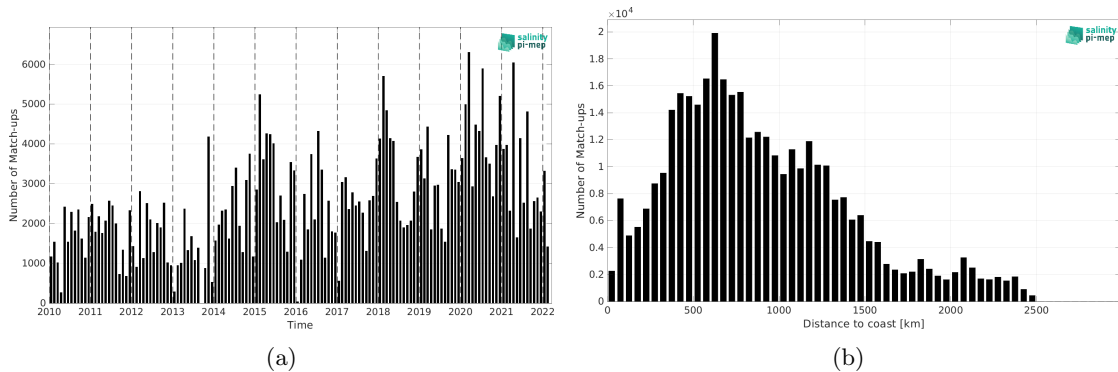
Figure 2: Number of match-ups between TSG (LEGOS-DM) and SMOS SSS L2Q v331 - No FLAG (CMEMS-CATDS-CPDC) SSS as a function of time (a) and as function of the distance to coast (b) over the North Pacific Ocean Pi-MEP region and for the full satellite product period.
