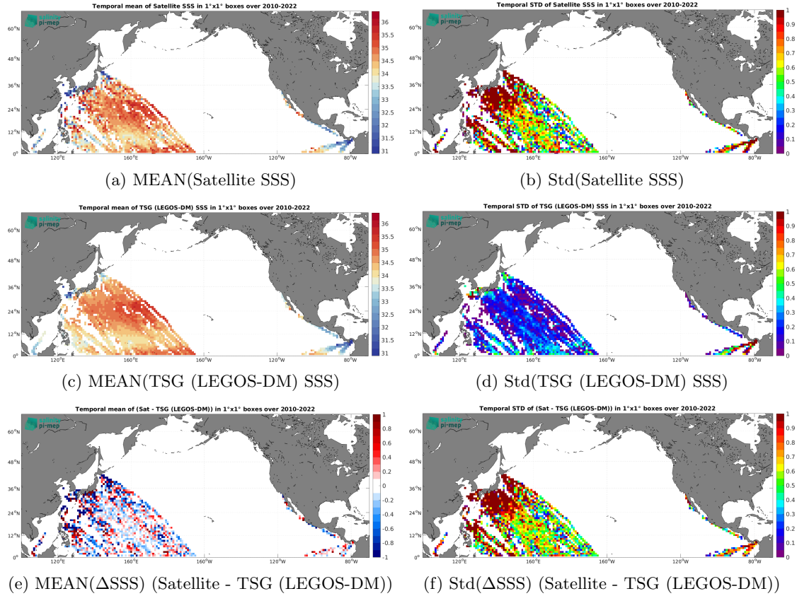
Figure 7: Temporal mean (left) and Std (right) of SSS from SMOS SSS L2Q v331 - No FLAG (CMEMS-CATDS-CPDC) (top), TSG (LEGOS-DM) (middle), and of \Delta\text{SSS} (Satellite - TSG (LEGOS-DM)). Only match-up pairs are used to generate these maps.
