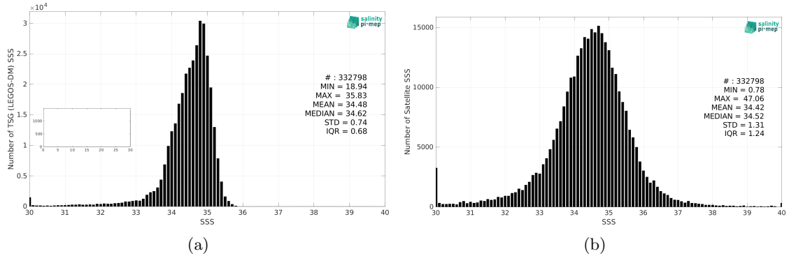
Figure 2: Histograms of SSS from TSG (LEGOS-DM) (a) and SMOS SSS L2Q v331 - No FLAG (CMEMS-CATDS-CPDC) (b) considering all match-up pairs per bins of 0.1 over the North Pacific Ocean Pi-MEP region and for the full satellite product period.
