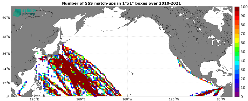
Figure 4: Number of SSS match-ups between TSG (LEGOS-DM) SSS and the SMOS SSS L2Q v331 - No FLAG (CMEMS-CATDS-CPDC) SSS product for the North Pacific Ocean Pi-MEP region over 1^\circ \times 1^\circ boxes and for the full satellite product period.
