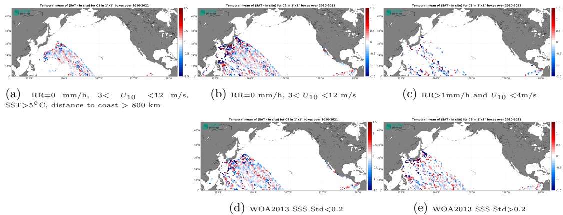
Figure 12: Temporal mean gridded over spatial boxes of size 1^\circ \times 1^\circ of \Delta SSS (SMOS SSS L2Q v331 - No FLAG (CMEMS-CATDS-CPDC) - TSG (LEGOS-DM)) for 5 different subdatasets corresponding to:RR=0 mm/h, 3 < U_{10} < 12 m/s, SST >5^\circ\text{C} , distance to coast > 800 km (a), RR=0 mm/h, 3 < U_{10} < 12 m/s (b), RR >1 mm/h and U_{10} < 4 m/s (c), WOA2013 SSS Std <0.2 (d), WOA2013 SSS Std >0.2 (e).
