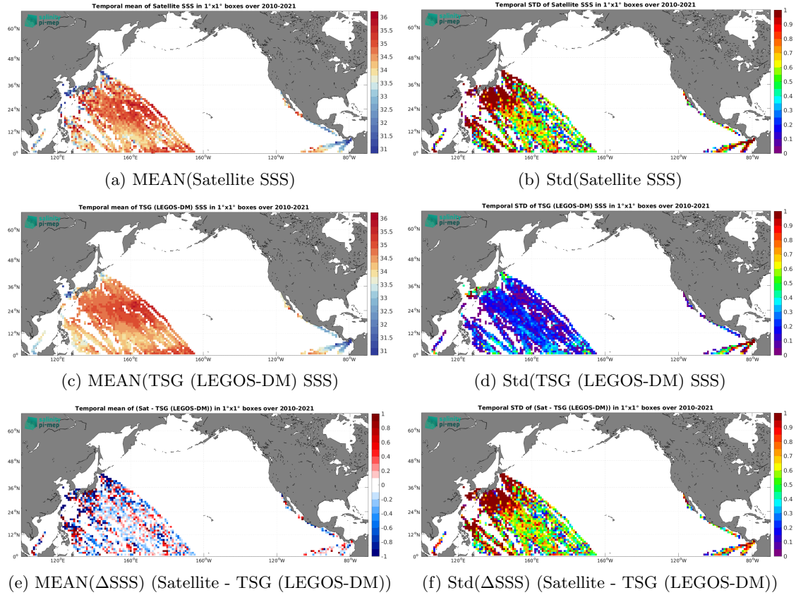
Figure 6: Temporal mean (left) and Std (right) of SSS from SMOS SSS L2Q v331 - No FLAG (CMEMS-CATDS-CPDC) (top), TSG (LEGOS-DM) ( in situ ) (middle), and of \Delta\text{SSS} (Satellite - TSG (LEGOS-DM)). Only match-up pairs are used to generate these maps.
