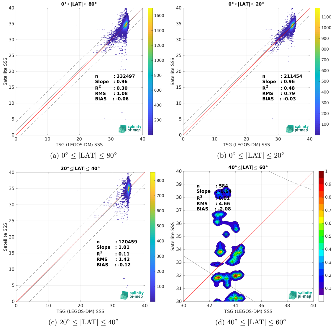
Figure 9: Contour maps of the concentration of SMOS SSS L2Q v331 - No FLAG (CMEMS-CATDS-CPDC) SSS (y-axis) versus TSG (LEGOS-DM) SSS (x-axis) at match-up pairs for different latitude bands. For each plot, the red line shows x=y . The black thin and dashed lines indicate a linear fit through the data cloud and the \pm 95\% confidence levels, respectively. The number match-up pairs n , the slope and R^2 coefficient of the linear fit, the root mean square (RMS) and the mean bias between satellite and in situ data are indicated for each latitude band in each plots.
