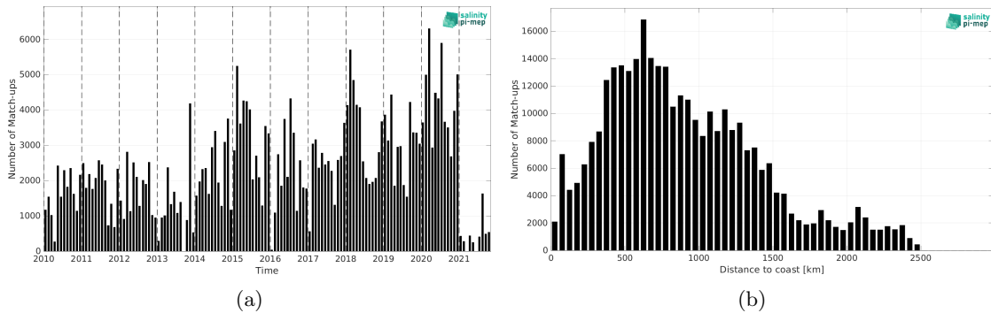
Figure 1: Number of match-ups between TSG (LEGOS-DM) and SMOS SSS L2Q v331 - No FLAG (CMEMS-CATDS-CPDC) SSS as a function of time (a) and as function of the distance to coast (b) over the North Pacific Ocean Pi-MEP region and for the full satellite product period.
