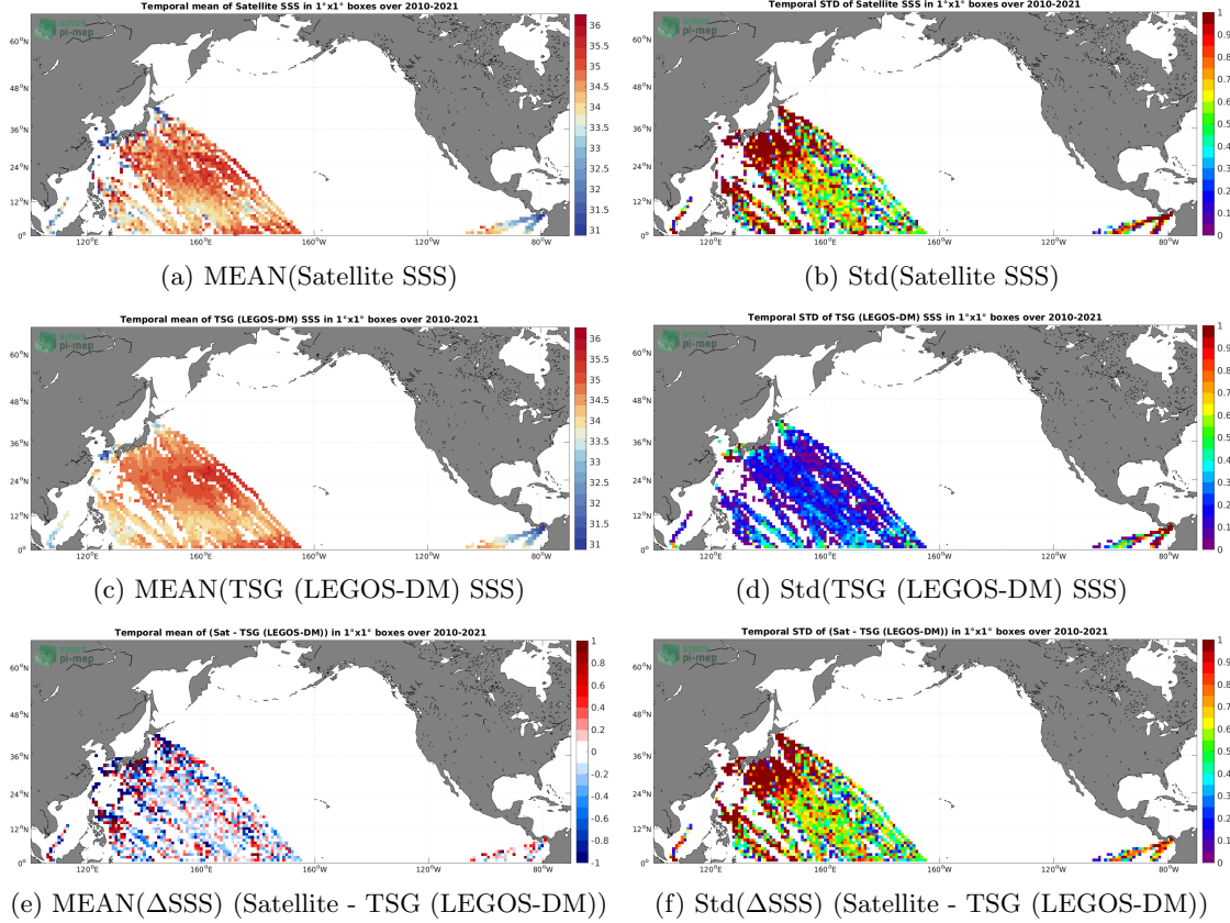
Figure 6: Temporal mean (left) and Std (right) of SSS from SMOS SSS L2Q v331 - No FLAG (CMEMS-CATDS-CPDC) (top), TSG (LEGOS-DM) (middle), and of \Delta\text{SSS} (Satellite - TSG (LEGOS-DM)). Only match-up pairs are used to generate these maps.
