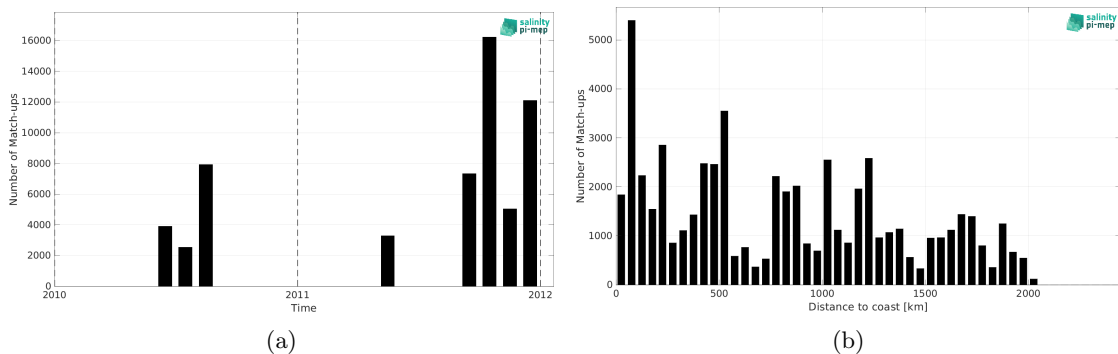
Figure 2: Number of match-ups between TSG (GOSUD-Sailing-ship) and SMOS SSS L2Q v331 - No FLAG (CMEMS-CATDS-CPDC) SSS as a function of time (a) and as function of the distance to coast (b) over the North Pacific Ocean Pi-MEP region and for the full satellite product period.
