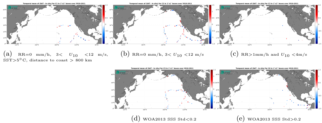
Figure 14: Temporal mean gridded over spatial boxes of size 1^\circ \times 1^\circ of \Delta SSS (SMOS SSS L2Q v331 - No FLAG (CMEMS-CATDS-CPDC) - TSG (GOSUD-Sailing-ship)) for 5 different sub-datasets corresponding to:RR=0 mm/h, 3 < U_{10} < 12 m/s, SST >5^\circ\text{C} , distance to coast > 800 km (a), RR=0 mm/h, 3 < U_{10} < 12 m/s (b), RR >1 mm/h and U_{10} < 4 m/s (c), WOA2013 SSS Std <0.2 (d), WOA2013 SSS Std >0.2 (e).
