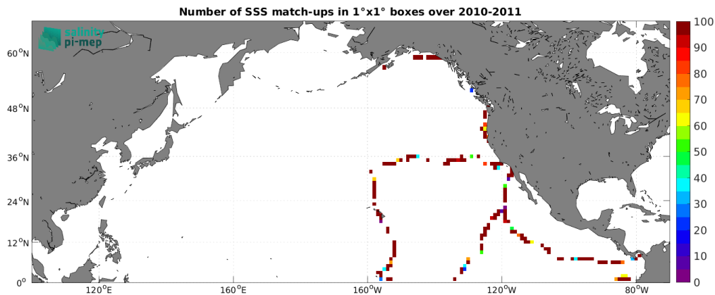
Figure 5: Number of SSS match-ups between TSG (GOSUD-Sailing-ship) SSS and the SMOS SSS L2Q v331 - No FLAG (CMEMS-CATDS-CPDC) SSS product for the North Pacific Ocean Pi-MEP region over 1^\circ \times 1^\circ boxes and for the full satellite product period.
