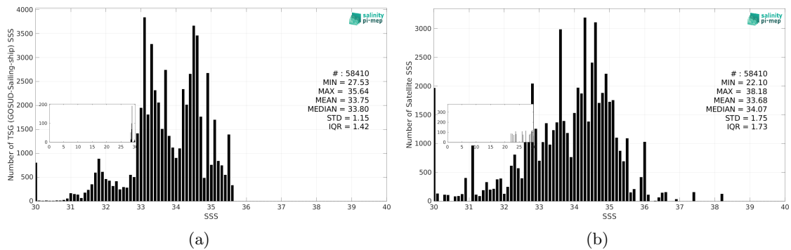
Figure 3: Histograms of SSS from TSG (GOSUD-Sailing-ship) (a) and SMOS SSS L2Q v331 - No FLAG (CMEMS-CATDS-CPDC) (b) considering all match-up pairs per bins of 0.1 over the North Pacific Ocean Pi-MEP region and for the full satellite product period.
