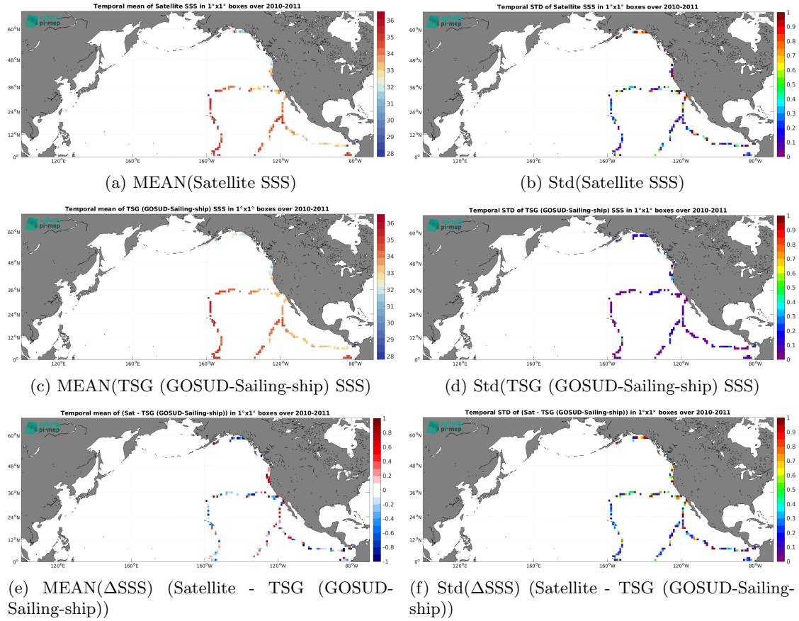
Figure 7: Temporal mean (left) and Std (right) of SSS from SMOS SSS L2Q v331 - No FLAG (CMEMS-CATDS-CPDC) (top), TSG (GOSUD-Sailing-ship) (middle), and of \Delta SSS (Satellite - TSG (GOSUD-Sailing-ship)). Only match-up pairs are used to generate these maps.
