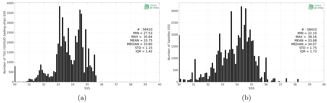
Figure 2: Histograms of SSS from TSG (GOSUD-Sailing-ship) (a) and SMOS SSS L2Q v331 - No FLAG (CMEMS-CATDS-CPDC) (b) considering all match-up pairs per bins of 0.1 over the North Pacific Ocean Pi-MEP region and for the full satellite product period.
