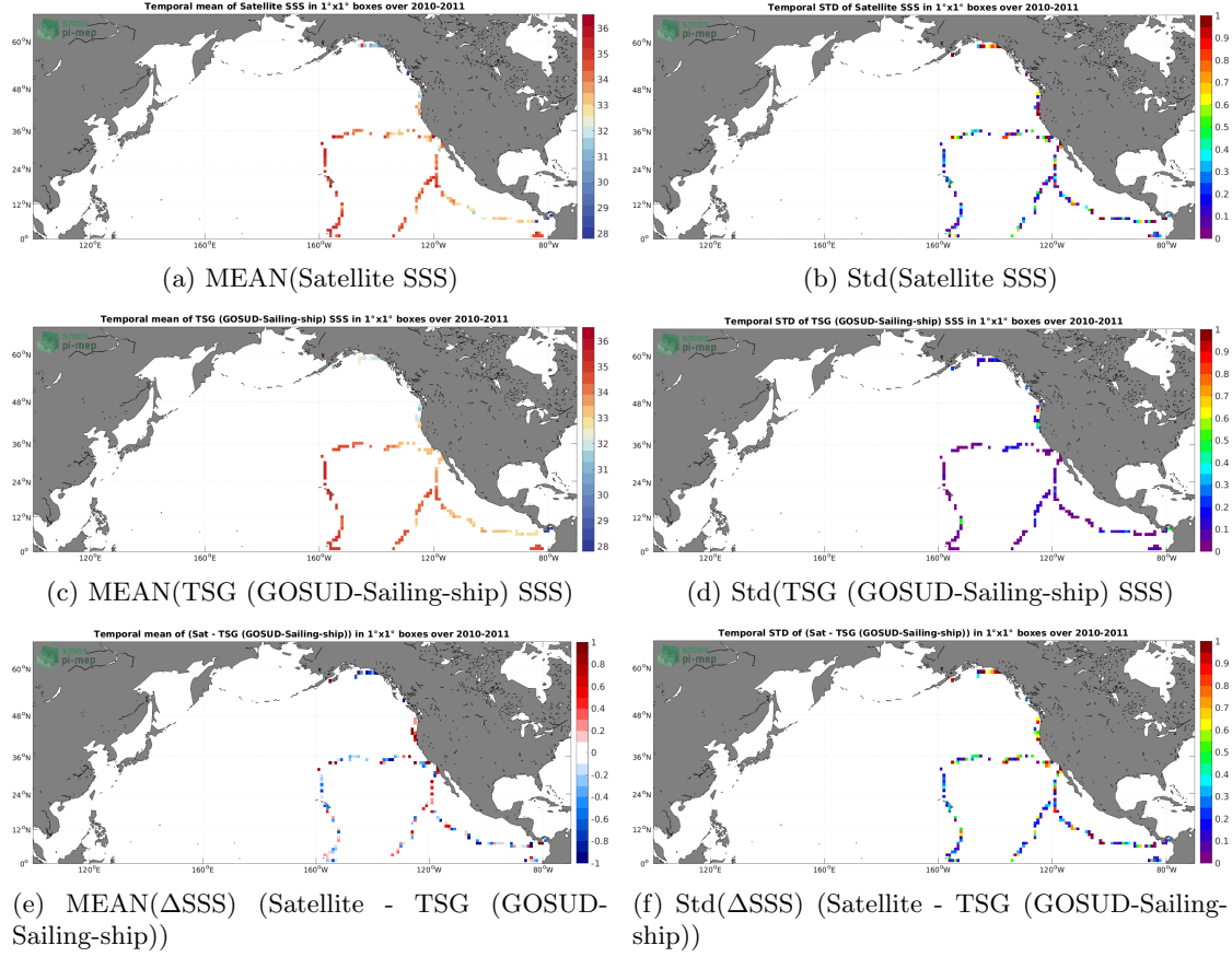
Figure 6: Temporal mean (left) and Std (right) of SSS from SMOS SSS L2Q v331 - No FLAG (CMEMS-CATDS-CPDC) (top), TSG (GOSUD-Sailing-ship) (middle), and of \Delta SSS (Satellite - TSG (GOSUD-Sailing-ship)). Only match-up pairs are used to generate these maps.
