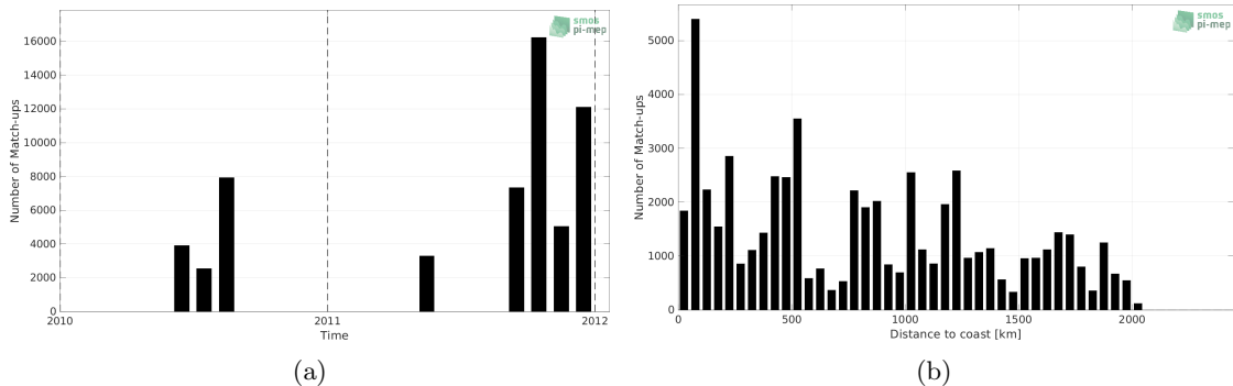
Figure 1: Number of match-ups between TSG (GOSUD-Sailing-ship) and SMOS SSS L2Q v331 - No FLAG (CMEMS-CATDS-CPDC) SSS as a function of time (a) and as function of the distance to coast (b) over the North Pacific Ocean Pi-MEP region and for the full satellite product period.
