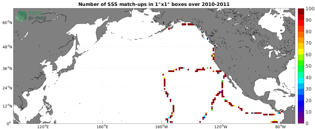
Figure 4: Number of SSS match-ups between TSG (GOSUD-Sailing-ship) SSS and the SMOS SSS L2Q v331 - No FLAG (CMEMS-CATDS-CPDC) SSS product for the North Pacific Ocean Pi-MEP region over 1^\circ \times 1^\circ boxes and for the full satellite product period.
