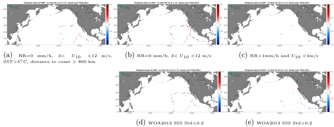
Figure 12: Temporal mean gridded over spatial boxes of size 1^\circ \times 1^\circ of \Delta SSS (SMOS SSS L2Q v331 - No FLAG (CMEMS-CATDS-CPDC) - TSG (GOSUD-Sailing-ship)) for 5 different sub-datasets corresponding to:RR=0 mm/h, 3 < U_{10} < 12 m/s, SST >5^\circ\text{C} , distance to coast > 800 km (a), RR=0 mm/h, 3 < U_{10} < 12 m/s (b), RR >1 mm/h and U_{10} < 4 m/s (c), WOA2013 SSS Std <0.2 (d), WOA2013 SSS Std >0.2 (e).
